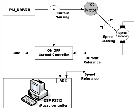
Fig. 2: Block diagram of proposed system.
