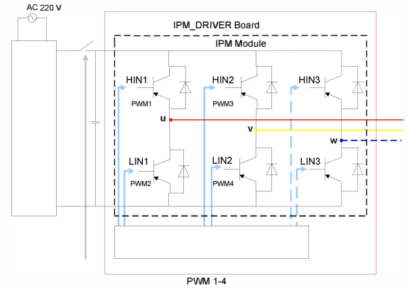
Fig. 3: Equivalent circuit of the IPM.
