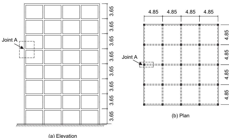
FIGURE 1 Eight-story frame building located in the western part of Canada (dimensions in meters).
