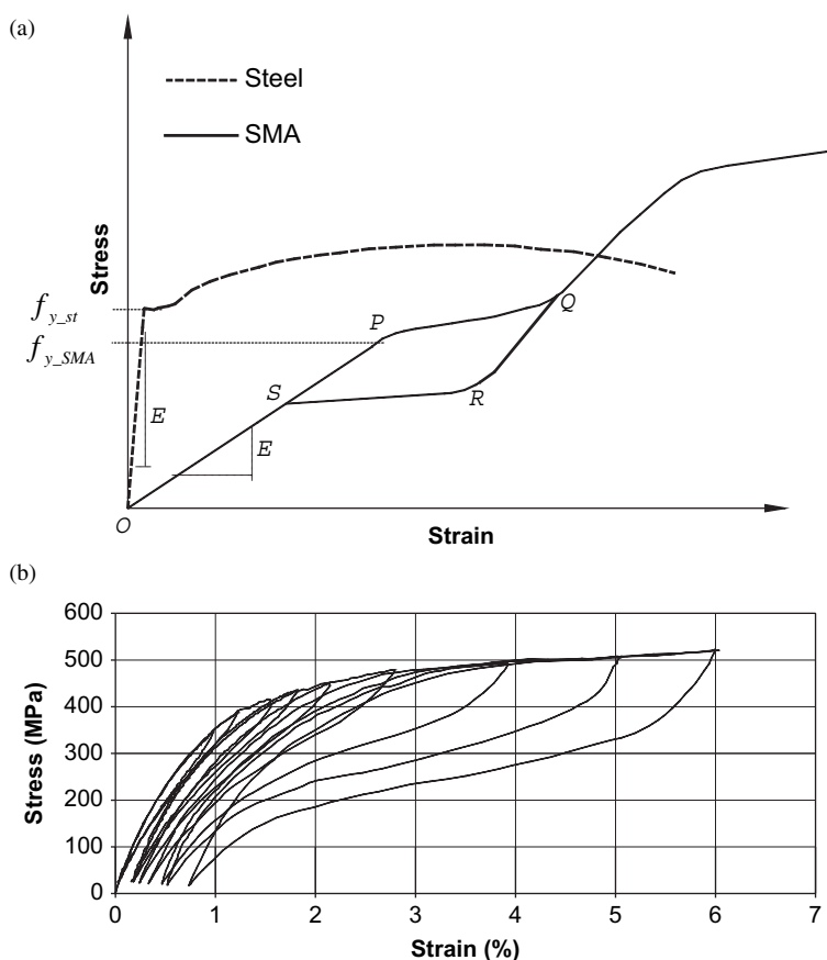
FIGURE 5 (a) Typical stress-strain behavior of SE SMA and steel; and (b) experimental cyclic tensile strength of SE SMA rebar within couplers.
