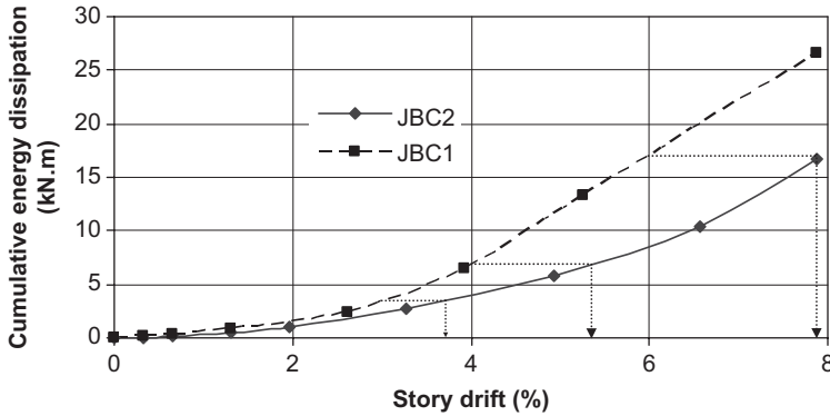
FIGURE 11 Cumulative energy dissipation-story drifts relationship of specimens JBC-1 and JBC-2.
