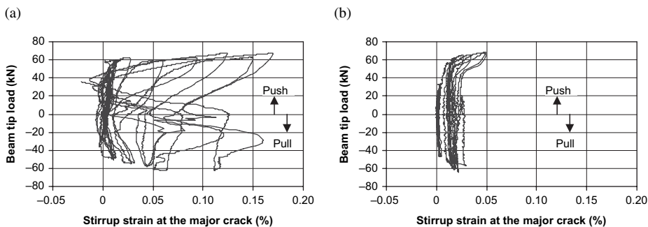
FIGURE 15 Strains in transverse reinforcement at the location of major crack of specimens: (a) JBC-1; and (b) JBC-2.
