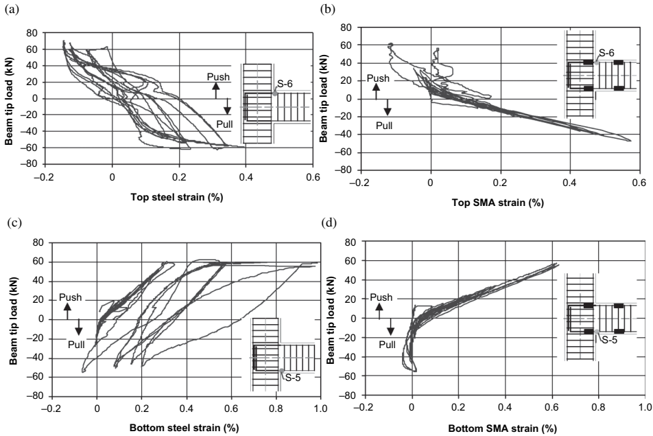
FIGURE 14 Strains in main longitudinal reinforcements at the column face of joint specimens: (a) top rebar of JBC-1; (b) top rebar of JBC-2; (c) bottom rebar of JBC-1; and (d) bottom rebar of JBC-2.
