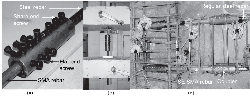
FIGURE 4 (a) Coupler used in JBC-2; (b) test setup of coupler in universal testing machine; and (c) reinforcement caging of JBC-2.
