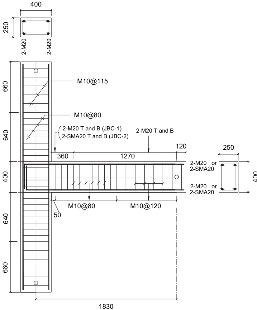
FIGURE 2 Reinforcement details of specimens JBC-1 and JBC-2 (all dimensions in mm).
