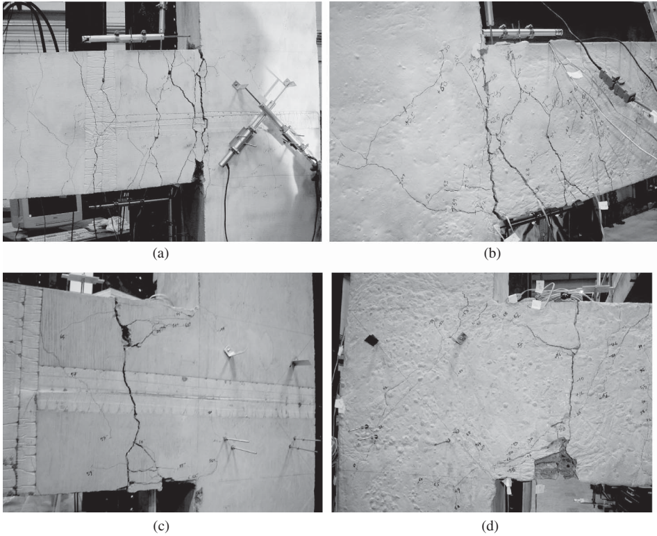
FIGURE 9 Crack pattern of specimens after being subjected to cycles up to 72 mm: (a) front face of JBC-1; (b) rear face of JBC-1; (c) front face of JBC-2; and (d) rear face of JBC-2.
