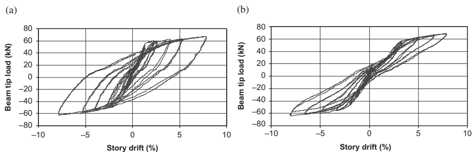
FIGURE 8 Beam tip load-story drift relationship of specimens: (a) JBC-1; and (b) JBC-2.
