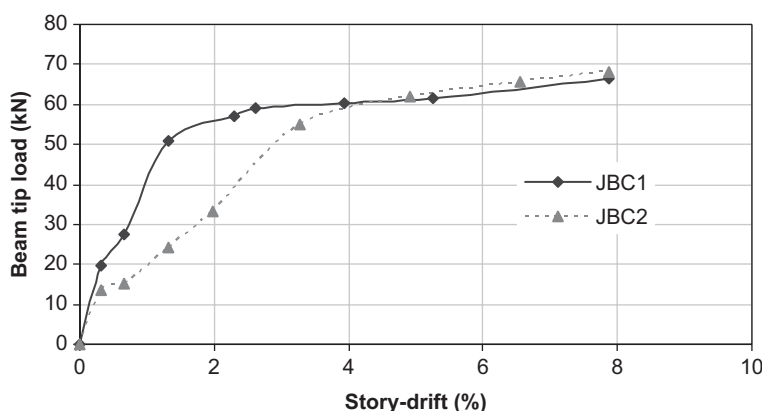
FIGURE 10 Beam tip-load versus story drift envelope of the tested specimens JBC-1 and JBC-2.
