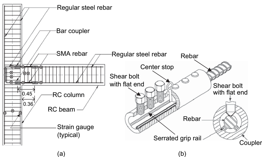
FIGURE 3 (a) Splice details of specimen JBC-2 and the positions of strain gauges; (b) regular single barrel screw-lock coupler for connecting SMA rebar with regular steel rebar (all dimensions in m).
