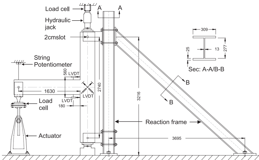
FIGURE 7 Test setup (all dimensions in mm).
