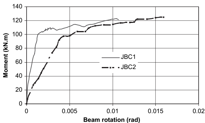
FIGURE 13 Beam moment versus rotation envelope of the tested specimens.
