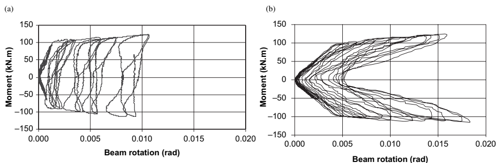
FIGURE 12 Beam moment-rotation plots at 180 mm away from the column face of specimens: (a) JBC-1; and (b) JBC-2.
