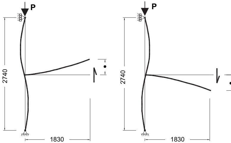
FIGURE 6 Typical deflected shape of specimen under reversed cycle of beam tip displacement.
