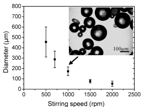
Figure 2. Diameter of catalyst-containing microcapsules as a function of stirring speed. Inset: optical microscopy image of microcapsules formed at 1000 rpm.
