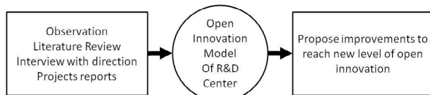
Fig. 4. Method
