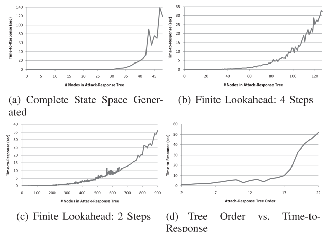
Fig. 6. Response system scalability analysis.
