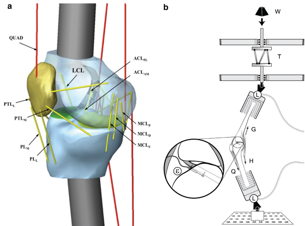
Fig. 1 Schematic diagrams of a the in silico knee model and b the in vitro test apparatus
