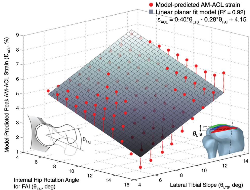
Fig. 3 In silico model predictions for peak anteromedial bundle–anterior cruciate ligament (AM-ACL) strain during a simulated jump landing: as the available range of hip internal rotation is reduced, the peak AM-ACL strain in the knee increases. The linear planar fit model (shown as the gray plane ) demonstrates how peak AM-ACL strain is predicted to be a function of both available axial hip range of motion and lateral tibial slope
