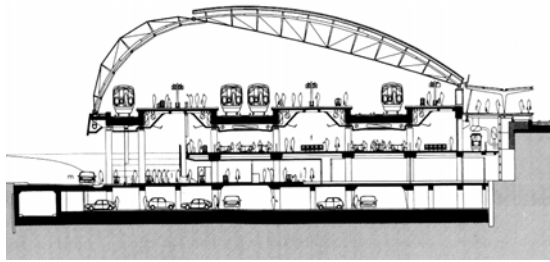
Figure 4. Waterloo International Terminal, London Cross section showing different levels of departure and arrival.
