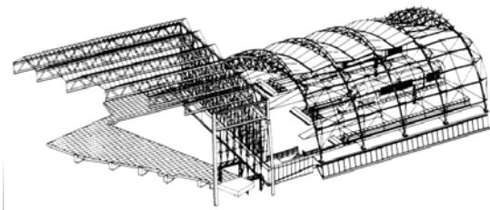
Figure 5. Waterloo International Terminal, London Dissected Perspective showing platform level on the third floor and its roof.
