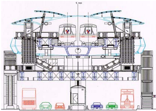
Figure 7. Cross section of a BTS station.
