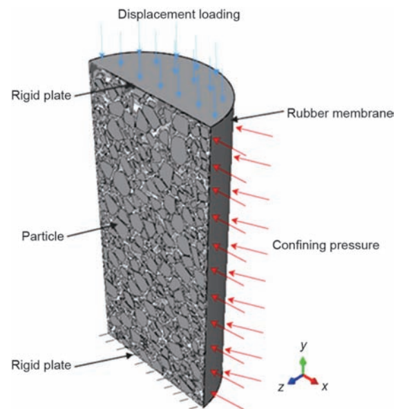
Fig. 3. Schematic diagram of a mesoscopic numerical shear test.
