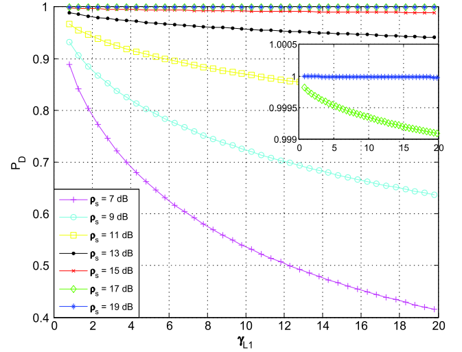
Fig. 1. P_D versus L1 for different values of \rho_s (from 7 dB to 19 dB).
