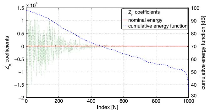
Fig. 3. KLT decomposition of the jammed interfered data in the GPS L1/Galileo E1 frequency band.
