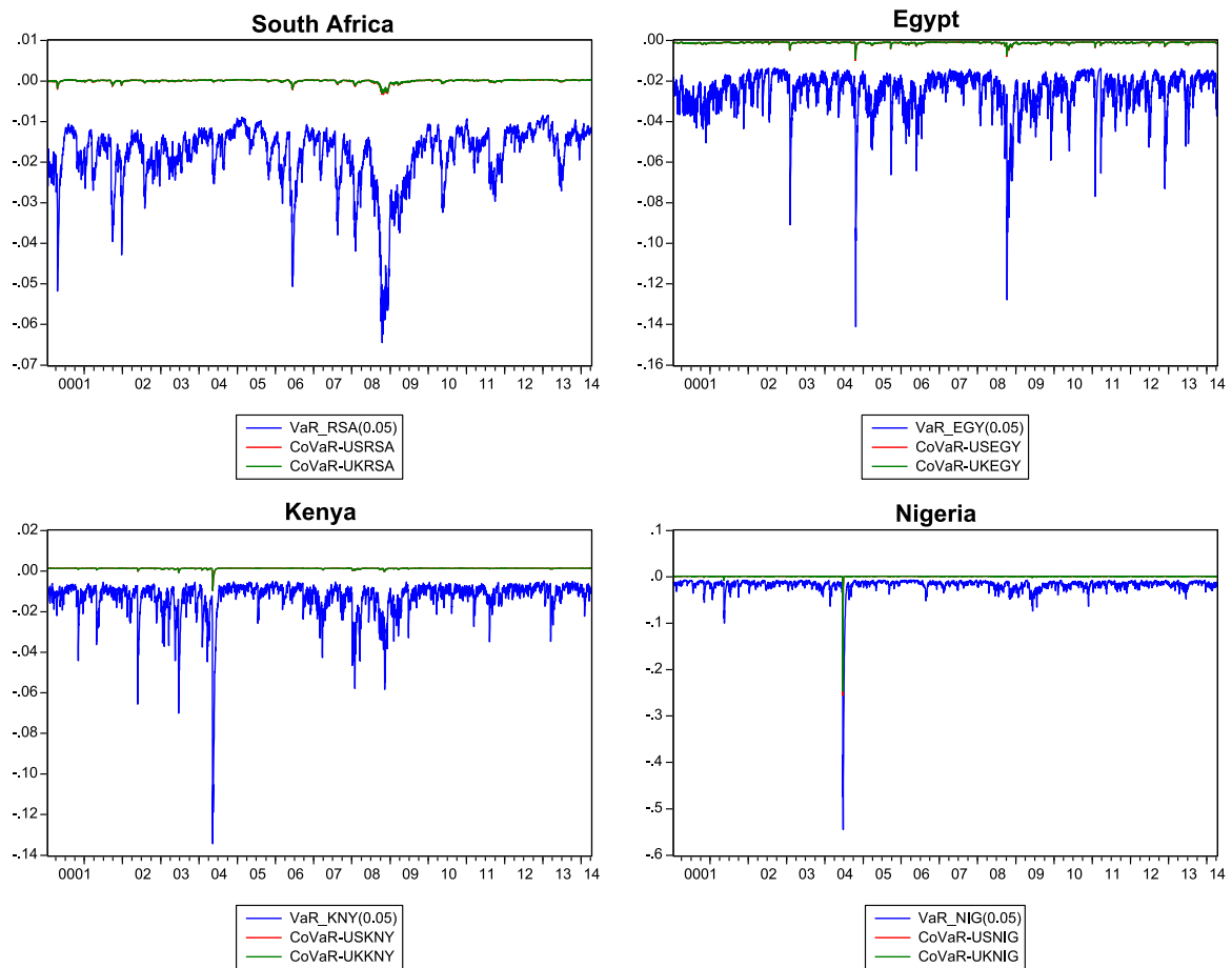
Fig. 3. Downside Value-at-Risk (VaR) and conditional Value-at-Risk (CoVaR) for African stock market returns. Notes: The blue line denotes time-varying 5%-Value-at-Risk. The red line denotes conditional Value-at-Risk for the US-related pairs. The green line denotes conditional Value-at-Risk for the UK-related pairs. African markets considered include South Africa (RSA), Egypt (EGY), Kenya (KNY) and Nigeria (NIG).
