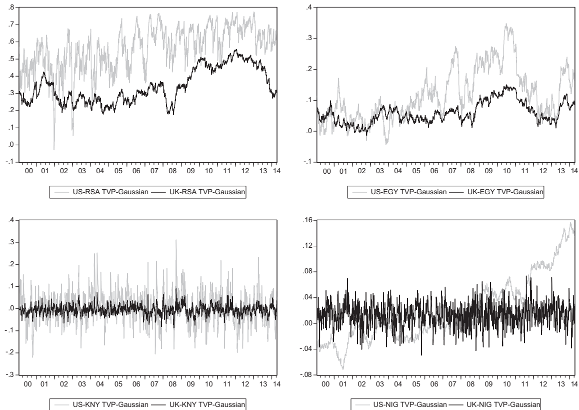
Fig. 1. Time-varying Gaussian Copula dependence of the USA, UK and African stock markets. Notes: The black line denotes the time-varying dependence between the UK stock market and African stock markets. The grey line denotes the time-varying dependence between the US stock market and African stock markets. African markets considered include South Africa (RSA), Egypt (EGY), Kenya (KNY) and Nigeria (NIG).
