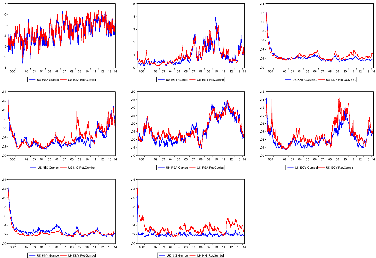
Fig. 2. Time-varying lower and upper tail dependence of the US and UK with African stock markets. Notes: The red line denotes the time-varying lower tail dependence implied by the TVP-rotated Gumbel copula. The blue line denotes the time-varying upper tail dependence implied by the TVP-Gumbel copula. African markets considered include South Africa (RSA), Egypt (EGY), Kenya (KNY) and Nigeria (NIG).
