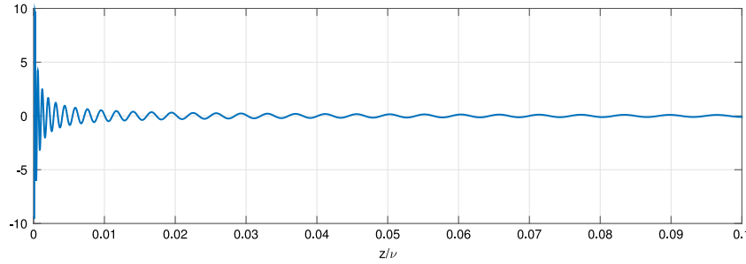
Fig. 1. The function L_{150}^{(4)}(z) is plotted as an example. The value of the parameter \nu (defined in (2)) is 610 in this particular case.
