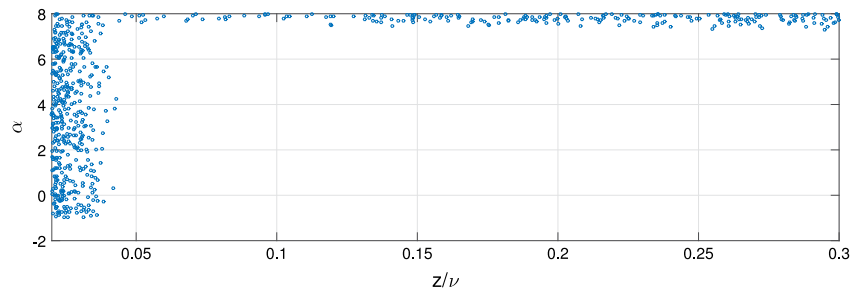
Fig. 3. Test of the performance of the Bessel-type expansion of Section 2.1.3. The points where the value of \epsilon in Eq. (40) is greater than 5 \cdot 10^{-12} are plotted.
