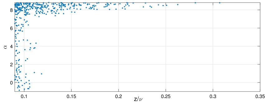
Fig. 4. Test of the performance of the Airy-type asymptotic expansion. The points where value of \epsilon in Eq. (40) is greater than 5 \cdot 10^{-12} are plotted.
