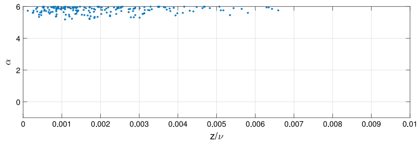
Fig. 2. Test of the performance of the simple Bessel-type expansion of Section 2.1.2. The points where the value of \epsilon in Eq. (40) is greater than 5 \cdot 10^{-12} are plotted.
