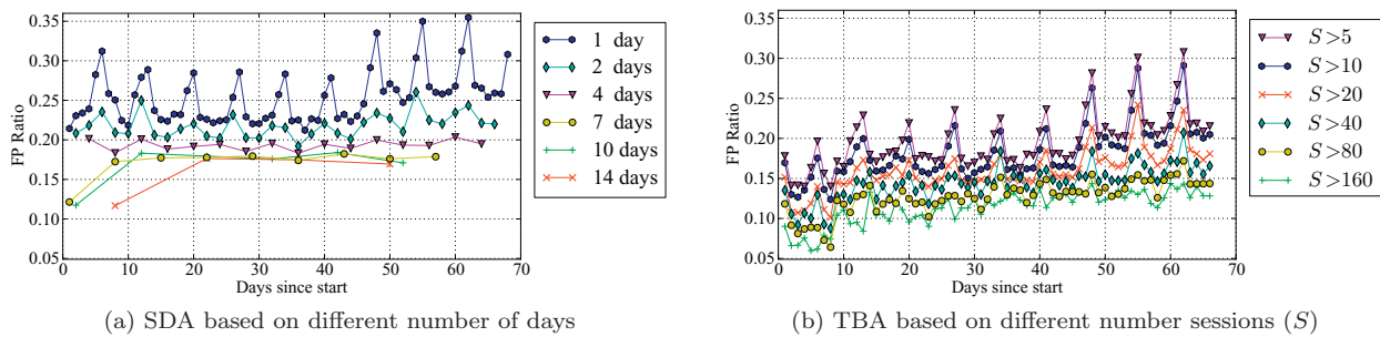
Fig. 12. Comparison of our different session aggregation approaches SDA and TBA using a J48 classifier.
