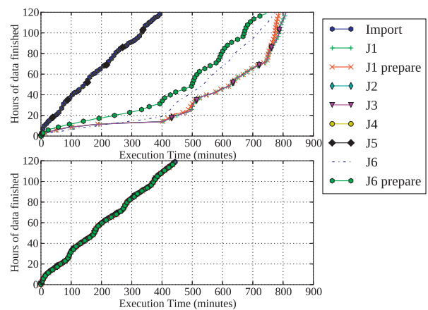
Fig. 8. DBStream task execution over time for FIFO and Shared scheduling.
