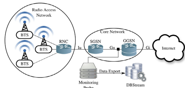
Fig. 9. Simplified overview of a 3G network including a monitoring system, e.g., METAWIN, and the data export to DBStream.
