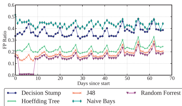
Fig. 10. FPR per day for selected classifiers.
