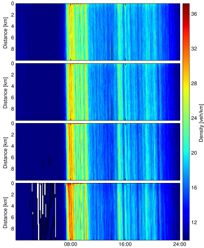
Fig. 7. Vehicular density heatmap, day-long M30 trace. Plots refer to lanes from right to left (bottom to top). Figure best viewed in color. (For interpretation of the references to color in this figure legend, the reader is referred to the web version of this article.)
