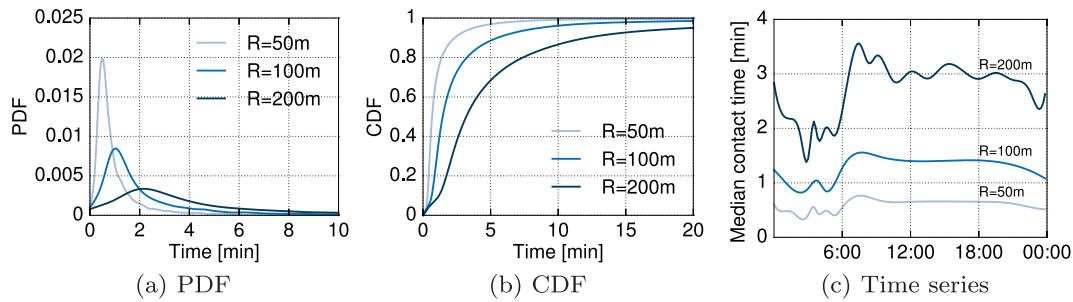
Fig. 17. Vehicle-to-vehicle contact duration on M30, under different values of the communication range R . (a) Time-aggregate PDF. (b) Time-aggregate CDF. (c) Time series, over 24 h.
