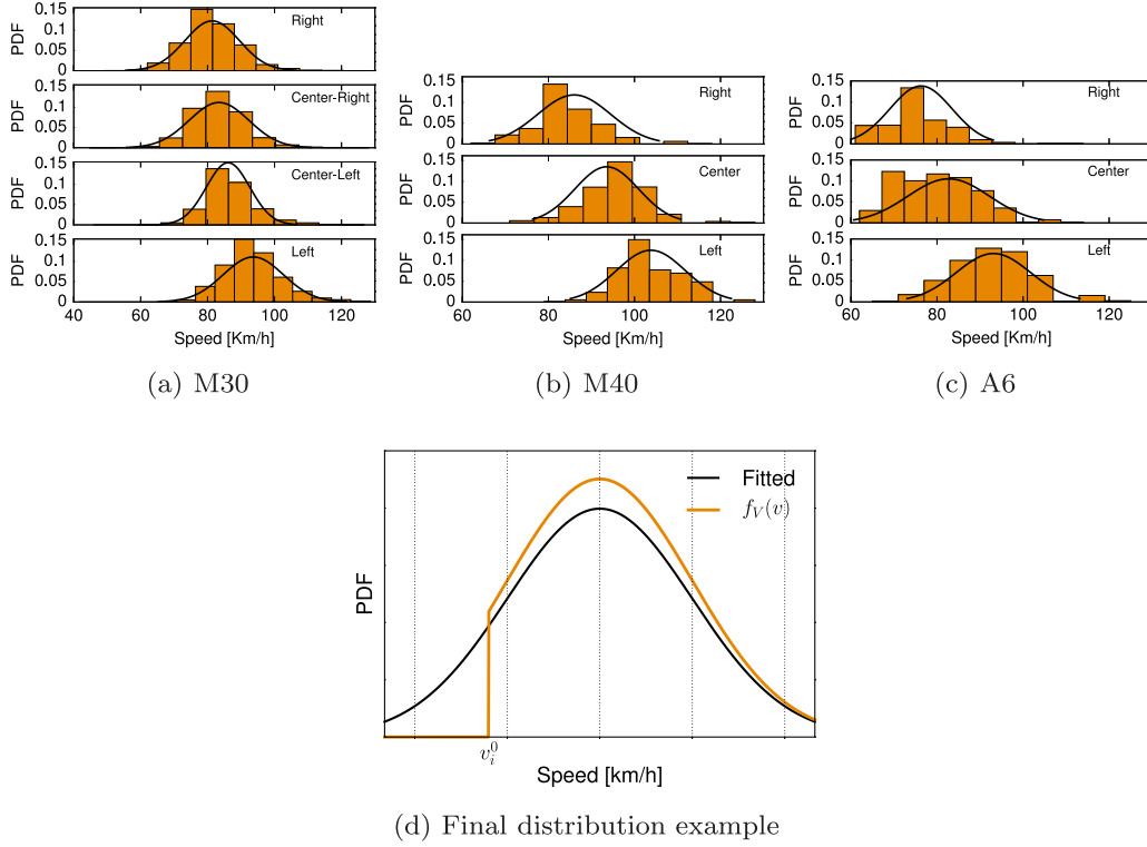
Fig. 5. Calculation of the maximum desired speed v_i^{max} . (a),(b),(c) Empirical and fitted distributions of the free flow speed on each lane of M30, M40 and A6, respectively. (d) Example of per-vehicle truncation and normalization of the fitted distribution, so that only values larger than the initial speed v_i^0 are considered for v_i^{max} , \forall i .
