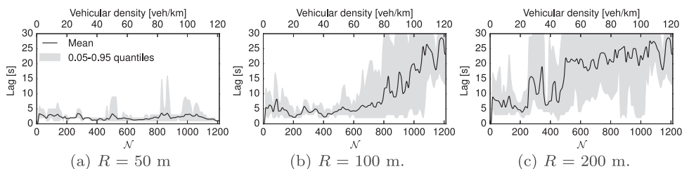
Fig. 14. Vehicular network average temporal stability versus the number of nodes \mathcal{N} , for different values of R .
