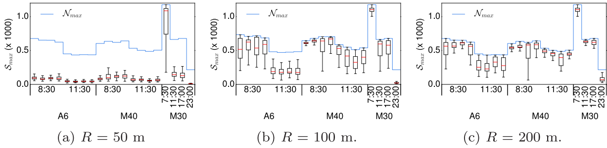
Fig. 9. The distribution of the largest component size, S_{max} , for different mobility traces, and varying R values.
