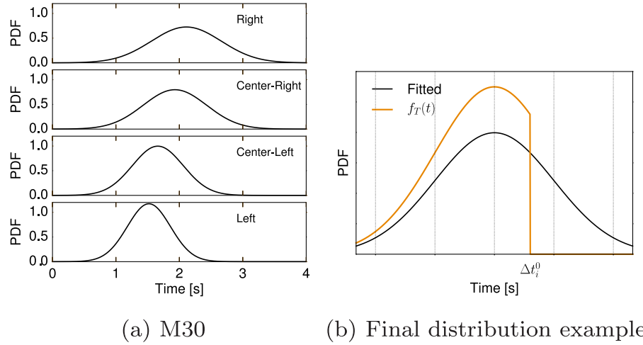
Fig. 6. Calculation of the minimum safe time headway \Delta t_i^{safe} . (a) Reference distributions of the typical safe time headway on each lane of M30, as inferred by the experimental flow, speed, and inter-arrival information contained in the traffic count dataset. (b) Example of per-vehicle truncation and normalization of the reference distribution, so that only values smaller than the initial inter-arrival time \Delta t_i^0 are considered for \Delta t_i^{safe} , \forall i .
