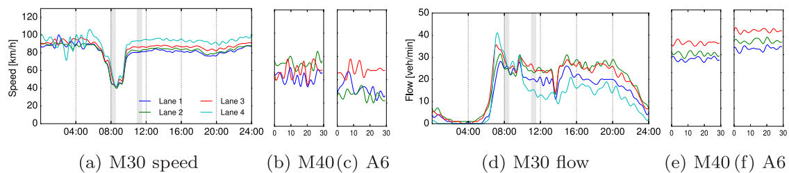
Fig. 2. Traffic count data overview. Per-lane speed (a) and in-flow (d) recorded during a full day on M30, and during two sample 30-min intervals (highlighted as gray-shaded in day-long plots) on M40 (b), (e) and A6 (c),(f).
