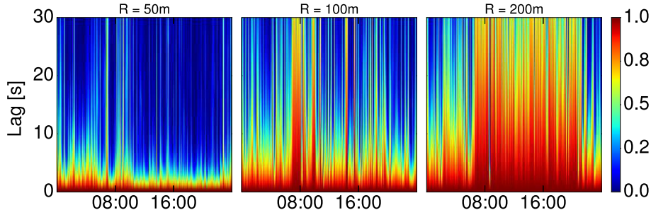
Fig. 13. Correlogram heatmap for S_{max} . Figure best viewed in color. (For interpretation of the references to color in this figure legend, the reader is referred to the web version of this article.)
