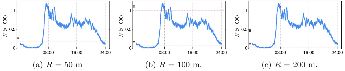
Fig. 11. Number of nodes \mathcal{N} , for different values of R . Critical thresholds are marked with A and B.
