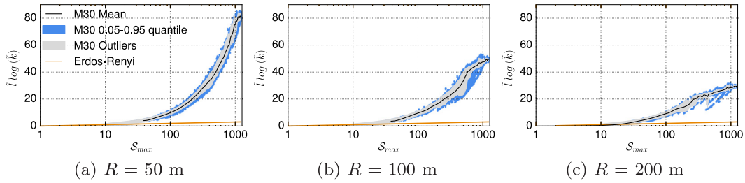
Fig. 15. Scaling properties of the average shortest path \bar{l} measured in the largest component C_{max} of the vehicular network, for different values of R . The result is compared to an Erdős–Rényi random graph of equivalent size S_{max} .
