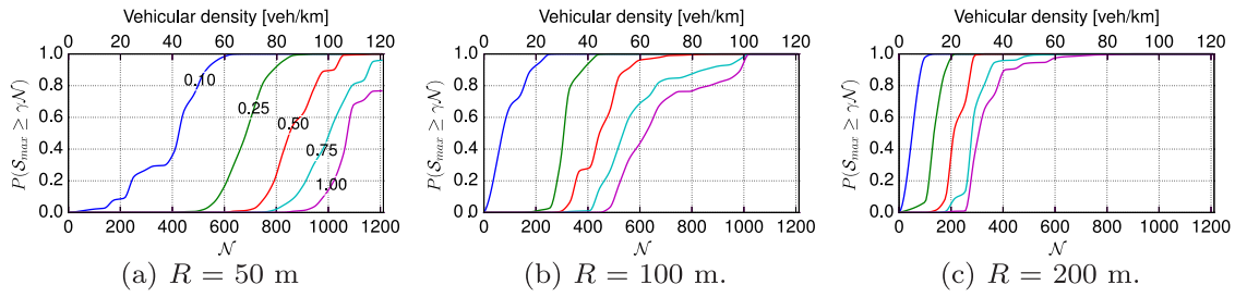
Fig. 12. Vehicular network average \gamma -availability versus the number of nodes \mathcal{N} , for different values of R .
