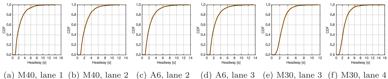
Fig. 3. Inter-arrival time CDF measured on May 12, 2010. Each plot refers a lane on M40 at 8:30 a.m. (a), (b), A6 at 11:30 a.m. (c), (d), and M30 at 11:30 a.m. (e),(f). Solid black lines represent the mixture model for each distribution.
