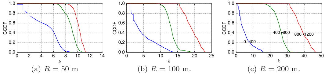
Fig. 16. CCDFs of the node degree k , for different values of R , separated according to S_{max} ranges.
