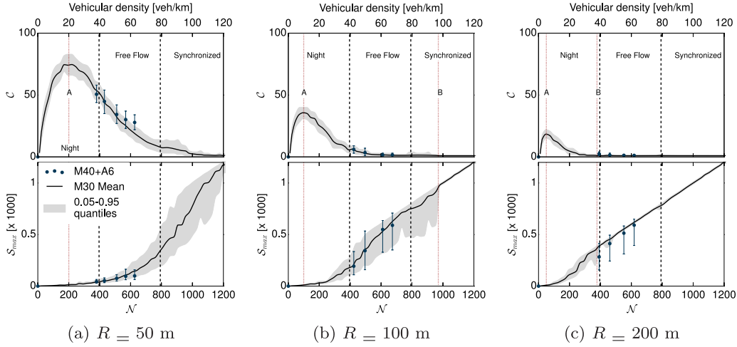
Fig. 10. C and S_{max} versus the number of nodes N for the M30, M40 and A6 datasets, for different R values. Blue points represent the average C with the 5th and 95th percentile when M30, M40 and A6 have valid N values. (For interpretation of the references to color in this figure legend, the reader is referred to the web version of this article.)
