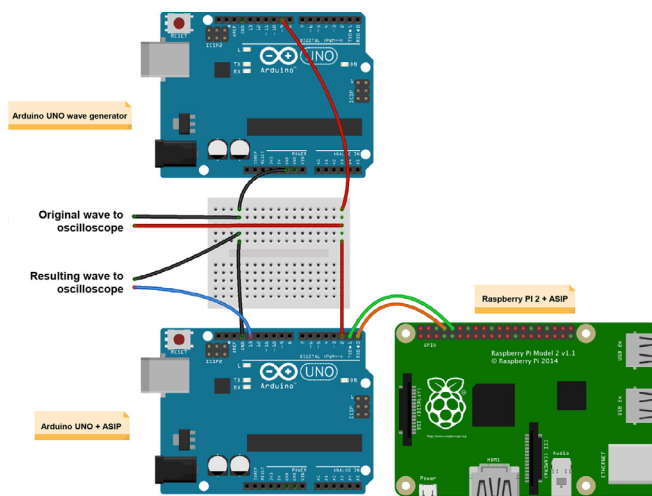
Fig. 4. Serial testing set-up.
