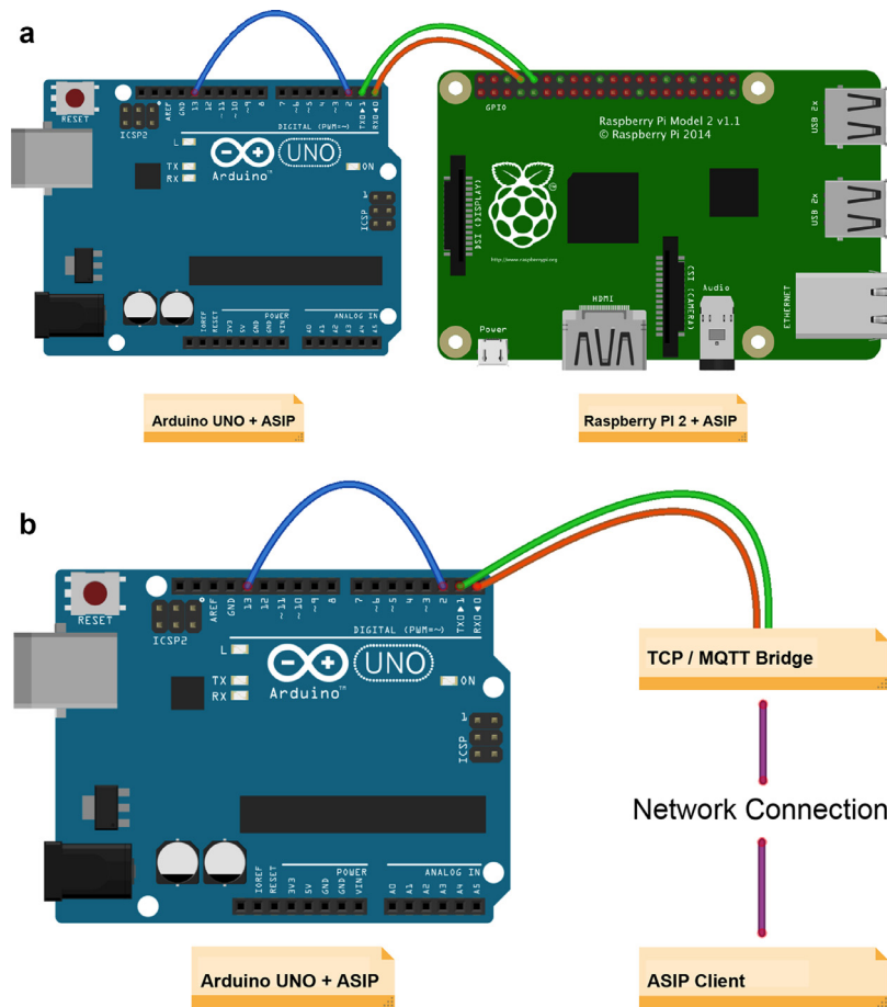
Fig. 7. The hardware set-ups used for latency testing: (a) serial connection and (b) TCP and MQTT connection.
