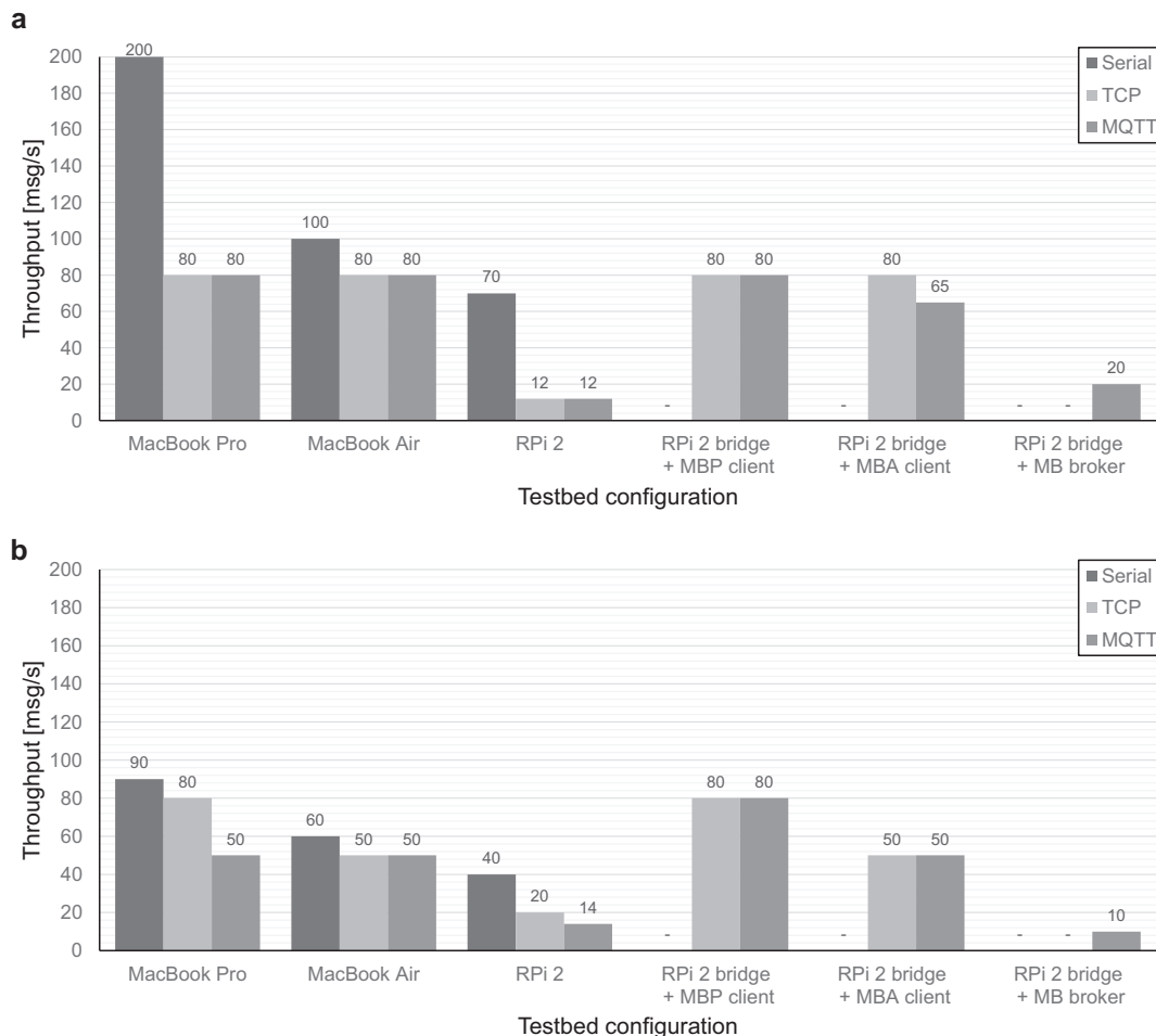
Fig. 6. Throughput for Java (a) and Python (b) clients with various testbed network configurations.
