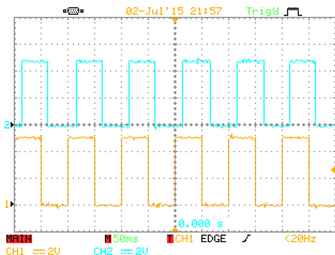
Fig. 5. Oscilloscope output.
