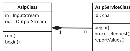
Fig. 1. ASIP simplified class diagram.
