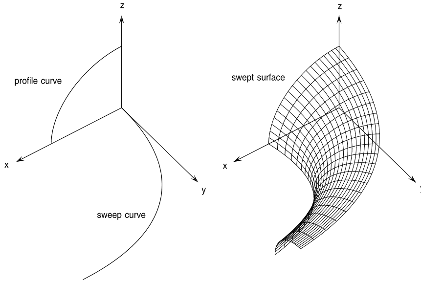
Fig. 6. The generalized conical swept surface (30) generated by a circular profile curve \mathbf{p}(u) in the (x, z) plane and a PH quintic sweep curve \mathbf{s}(v) in the (x, y) plane, with factors c_0 = 1 and c_1 = \frac{1}{2} in the scaling function (29).
