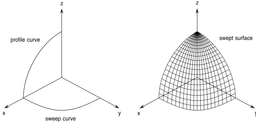
Fig. 1. The scaled-rotation surface defined by a circular arc in the (x, z) plane as the profile curve, and a cubic in the (x, y) plane as the sweep curve.
