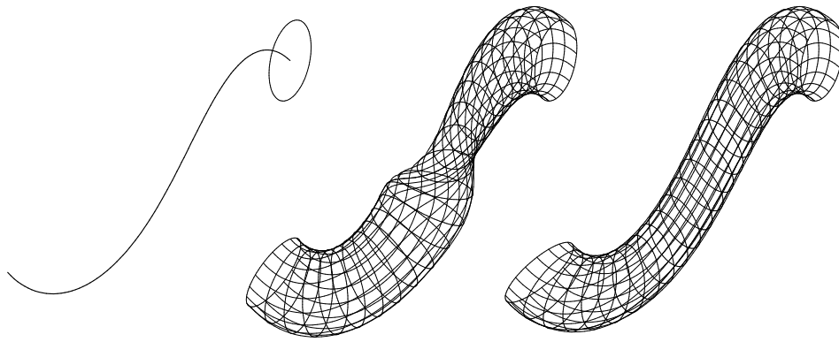
Fig. 8. The tubular surface generated by sweeping an ellipse profile curve along an RRMF quintic sweep curve (left). The profile curve lies in the sweep curve normal plane at each point, and within this plane it is oriented using either the Frenet frame (center) or the rotation-minimizing frame (right).
