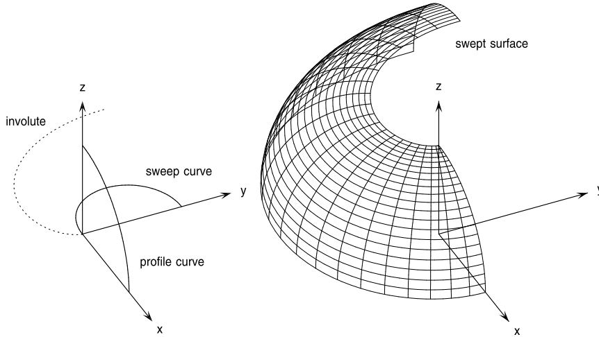
Fig. 5. Left: a circle arc in the (x, z) as the profile curve, and a PH quintic sweep curve in the (x, y) plane, together with its involute (the dotted curve). Right: the oriented-involute swept surface generated by these two curves.
