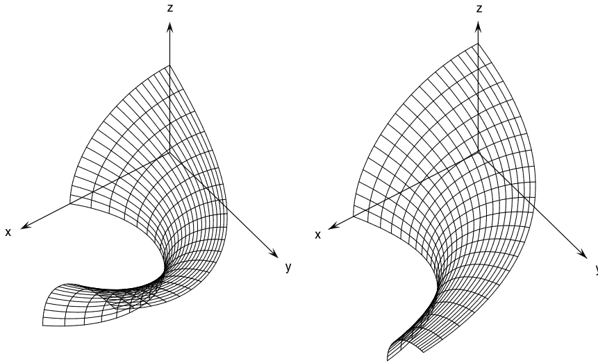
Fig. 7. Generalized conical swept surfaces generated by a circular profile curve \mathbf{p}(u) in the (x, z) plane and a PH quintic sweep curve \mathbf{s}(v) in the (x, y) plane, using the quadratic scaling function (33) with coefficients (c_0, c_1, c_2) = (1.0, 0.0, 1.0) on the left, and (c_0, c_1, c_2) = (1.25, 0.75, 0.50) on the right.
