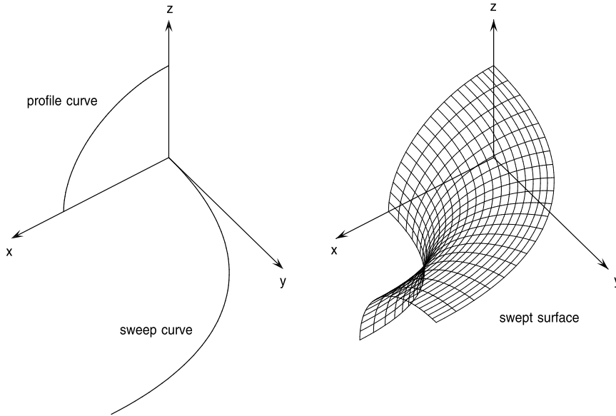
Fig. 2. The oriented-translation surface generated by a circular arc profile curve in the (x, z) plane, and a PH quintic sweep curve in the (x, y) plane.
