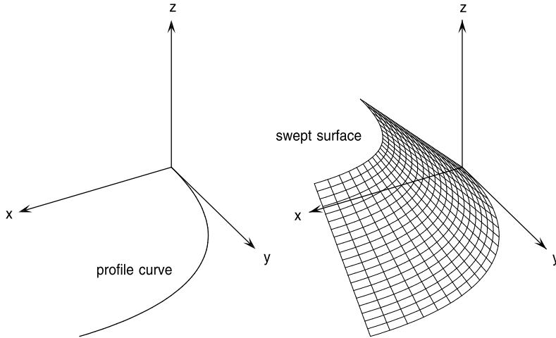
Fig. 3. The offset-translation swept surface (20) generated by a PH quintic profile curve \mathbf{p}(u) in the (x, y) plane and offset distance function d(v) = v .
