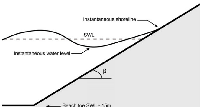
Fig. 5. Schematic of the idealised gravel beach profile used to generate the XBeach-G runup dataset.
