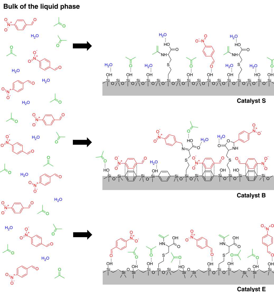
Fig. 2. Representation of the selective enrichment and the related formation of reactive enamine intermediates and inhibiting species in the pores of silica material, catalyst S, catalyst B containing benzene bridges and catalyst E containing ethane bridges.
