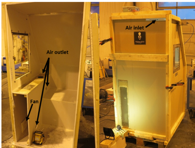
Fig. 1. Mockup of the toilet compartment in buses, seen from the front without door (left image) and with door (right image).
