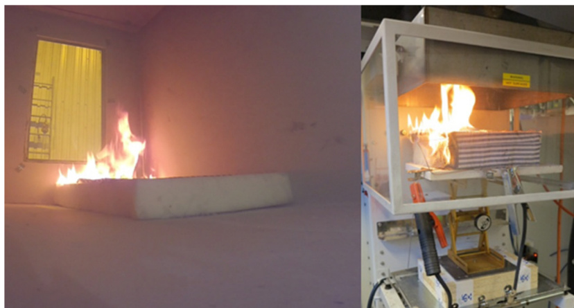
Fig. 7. Mattress fire source in the sleeping compartment mockup (left) and in the calorimeter setup (right).
