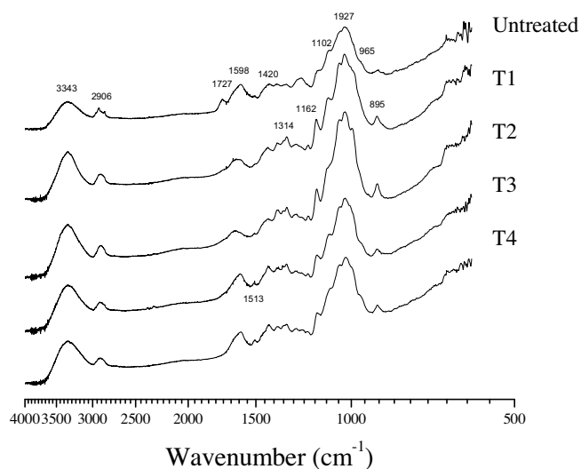
Fig. 5. ATR-FTIR spectra of untreated soybean straw (untreated) and after chemical treatments T1, T2, T3, and T4.
