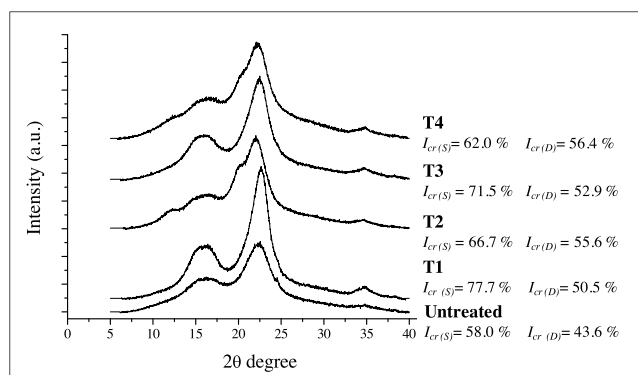
Fig. 3. X-ray diffractograms and crystalline index of untreated SS and treated SS samples (T1, T2, T3, and T4) as estimated by the Segal equation-XRD peak height ( I_{cr(S)} ) and by the XRD deconvolution method ( I_{cr(D)} ).
