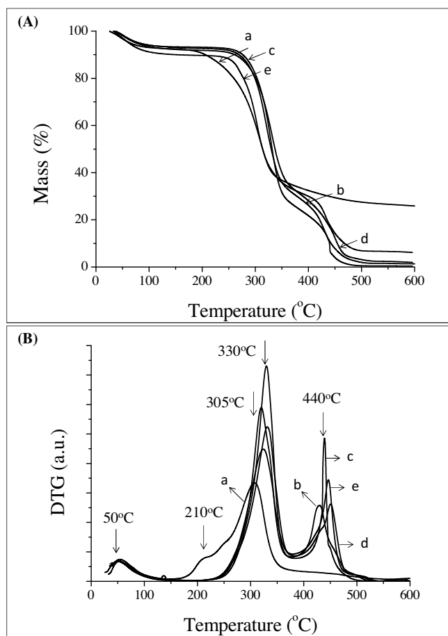
Fig. 4. (A) TGA and (B) DTG scans of (a) untreated soybean straw and soybean straw after chemical treatments (b) T1, (c) T2, (d) T3, and (e) T4, as described in Fig. 1.
