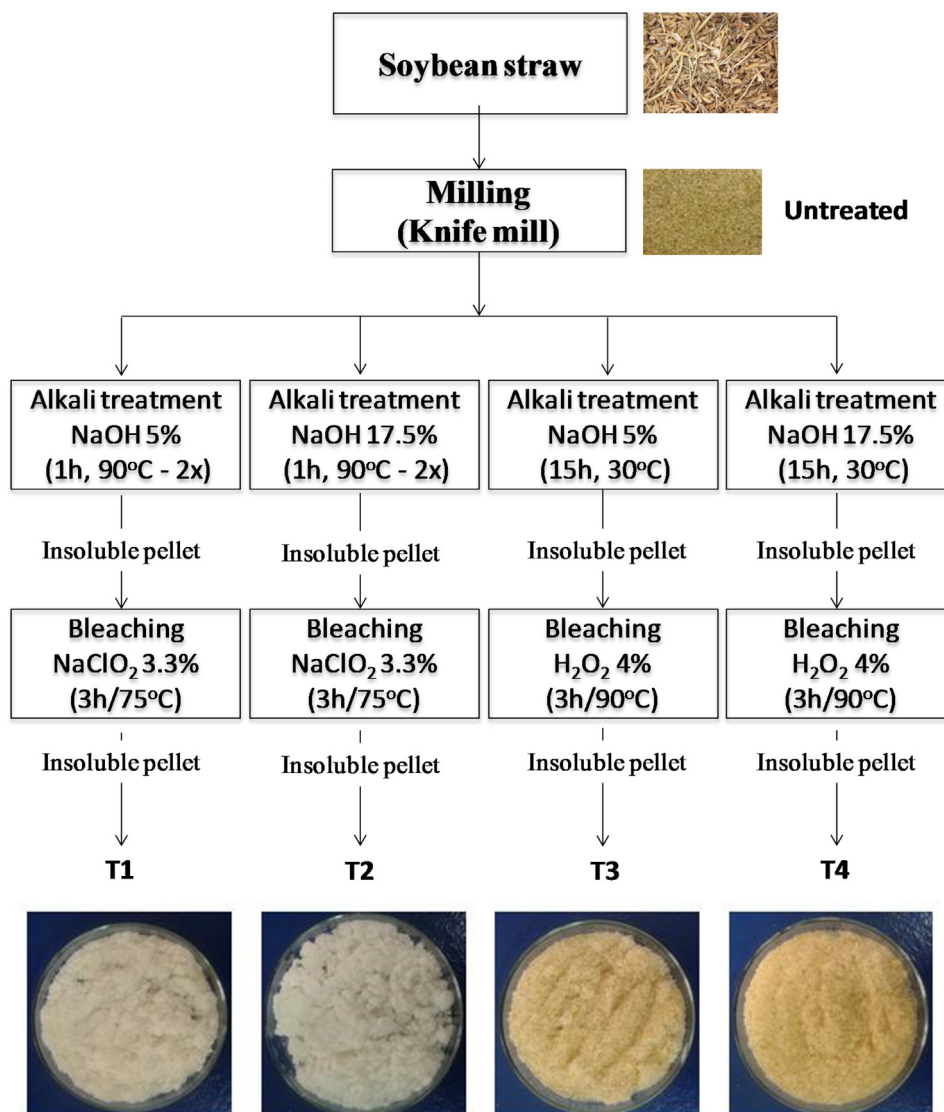
Fig. 1. Chemical pre-treatments of the soybean straw.
