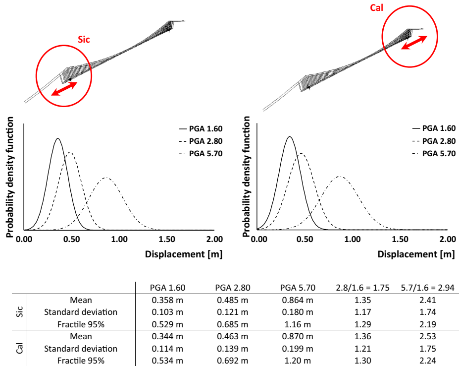
Fig. 9. Longitudinal displacement of the bridge deck at the expansion joints.
