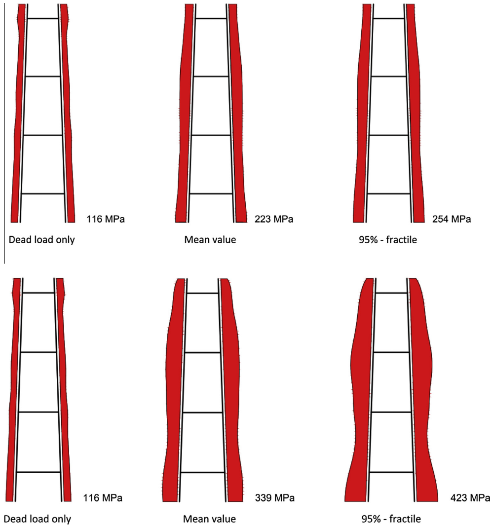
Fig. 14. Stress values in tower piers due to seismic load with PGA = 2.60 m/s 2 (top) and PGA = 5.70 m/s 2 (bottom).
