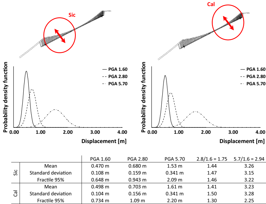
Fig. 11. Transverse displacement of the bridge deck at a quarter of the bridge.
