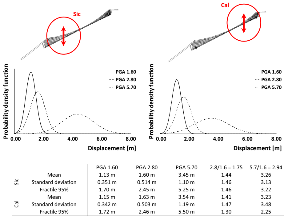
Fig. 12. Vertical displacement of the bridge deck at a quarter of the bridge.
