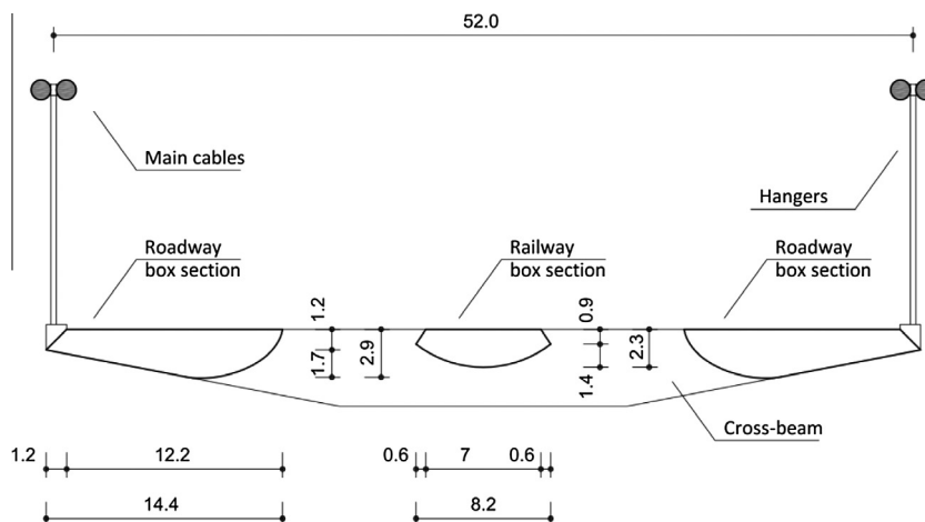
Fig. 2. Geometrical dimensions of the bridge-deck section (m).
