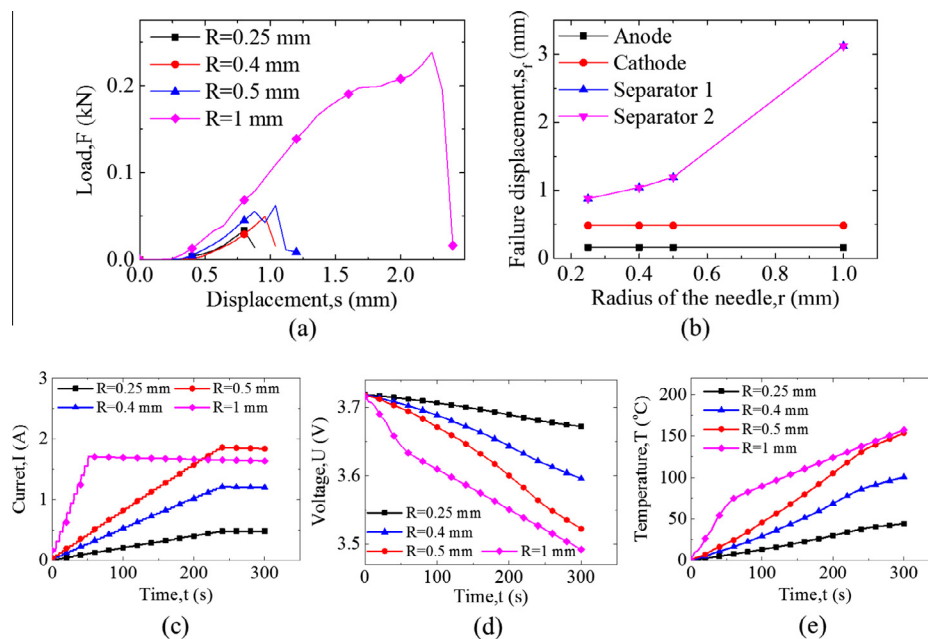
Fig. 6. Results of different nail sizes in penetration: (a) load–displacement curve, (b) relationship between failure displacement and shape, (c) current–time curve after a short circuit, (d) voltage–time curve after a short circuit, and (e) maximum increased temperature–time curve after a short circuit.
