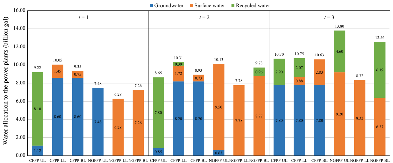
Fig. 5. Optimized water allocation from the different models over the three planning periods (CFPP: coal-fired power plant; NGFPP: natural gas-fired power plant; UL: upper-level model; LL: lower-level model; BL: bi-level model).
