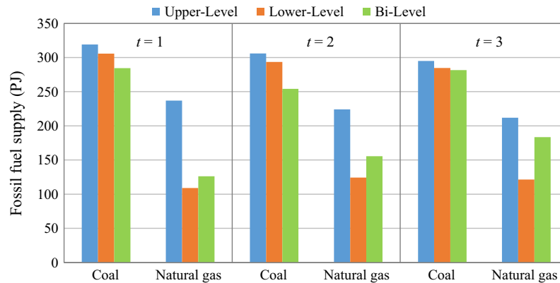
Fig. 3. Optimized fossil fuel supply during the three planning periods.
