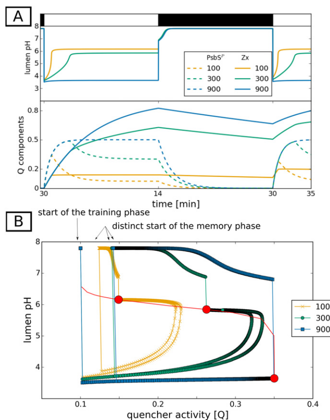
Fig. 5. Visualisation of luminal pH changes in the response to different light intensities. (A) Internal variables for three different light intensities. The upper panel shows how the ability of relaxing the luminal pH is lost with increasing light intensity. The bottom panel shows the dynamics of the quenching components (solid line for the relative zeaxanthin concentration, dashed line for the ratio of protonated PsbS). (B) The phase plane trajectories of the quenching variable (Q) and the luminal pH during the light memory protocol. The red line depicts stationary states calculated for different light intensities with three red circles marking the steady states for the three light intensities examined experimentally. The markers on the trajectories are set in regular intervals of 1 s to visualise the different time scales on which the system is operating.
