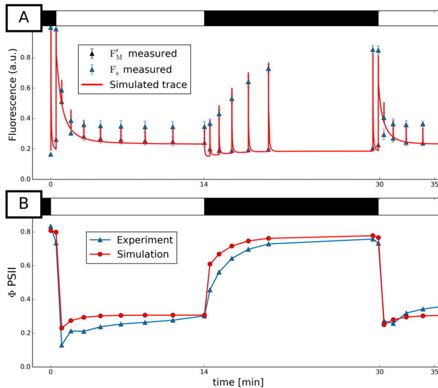
Fig. 6. (A) Measured and simulated fluorescence traces for Pothos exposed to light of 100 \mu\text{Em}^{-2}\text{s}^{-1} intensity. Minimal change into the parameter space of the model enabled reproducing all key features of the fluorescence dynamics. (B) Inhibitory effect of light on the photosynthetic activity (expressed in terms of maximal yield) is reproduced in our simulation.
