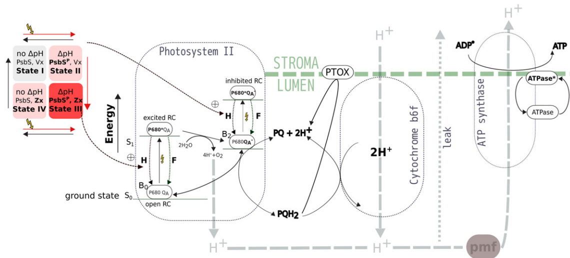
Fig. 3. Scheme of the components included in the simplified mathematical model. It contains a detailed description of internal processes occurring inside photosystem II (for more details of the four state description of PSII see the SI Text ) that are directly affected by the 4 state quencher. The plastoquinone pool is reduced by PSII, which also releases protons into the lumen by the oxygen evolving complex. PQ can be oxidised by cytochrome b6/f and PTOX. Oxidation by cyt b6/f is coupled to proton translocation from stroma to lumen. Protonation of the lumen drives the production of ATP through ATPase. ATPase is active in the light and inactive in the dark. Protons can also passively leak out of the thylakoid lumen.
