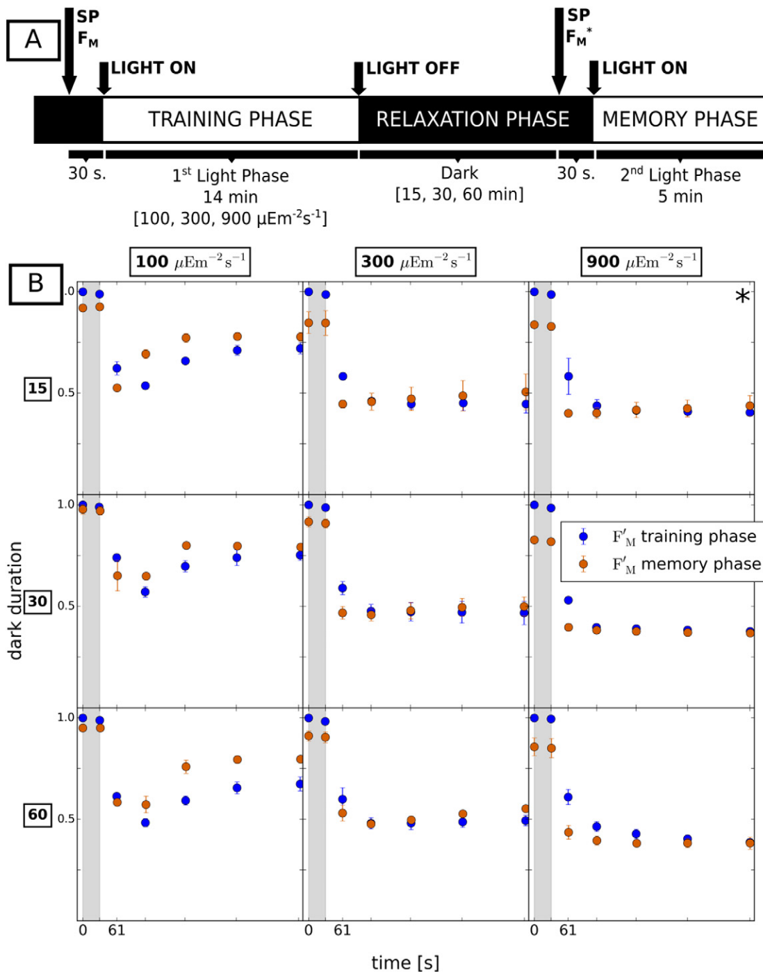
Fig. 1. (A) Design of the experiment. Dark adapted plants were exposed to a first saturating pulse of light (SP) from which physiological parameters such as maximal fluorescence ( F_M ) and photosynthetic yield ( \Phi\text{PSII} ) were derived. 30 s into darkness a second SP was applied, then the light was switched on for a fixed (training) period of 14 min. SPs were applied in a defined sequence (see Fig. S1), yielding maximal fluorescence ( F_M ). The training period was followed by a dark period, interrupted by six SP to follow the fluorescence relaxation dynamics. Subsequently, in the second (memory) period, the same illumination intensity as in the training period was applied. Each experiment was repeated three times for three light intensities (100, 300 and 900 \mu\text{Em}^{-2}\text{s}^{-1} ) and different relaxation times (15, 30 and 60 min). (B) Comparison of the first two F_M measurements taken in darkness and first five measurements in training phase (blue points) with the last two measurements taken in the relaxation phase and first five measurements in the second light phase (red points). The first measurement taken in the light (at 61 s) is lower in the memory phase than in the training phase, regardless of light intensity and time of relaxation. Error bars indicate standard deviations for three replicates except for the experiment marked with *, where the experiment was repeated eight times (see the SI Text for motivation).
