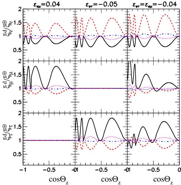
Fig. 3. Flavor ratios at the detector as a function of the zenith angle of the neutrino normalized to the expectation in the absence of NSI and for oscillation parameters at the best fit of the global analysis ( \sin^2 \theta_{12} = 0.305 , \sin^2 \theta_{13} = 0.0219 , \sin^2 \theta_{23} = 0.579 , and \delta_{CP} = 254^\circ ). For the left (central) [right] panels the only non-vanishing NSI parameters are \varepsilon_{e\mu} = 0.04 ( \varepsilon_{e\tau} = -0.05 ) [ \varepsilon_{e\mu} = \varepsilon_{e\tau} = -0.04 ]. The different curves correspond to different flavor composition at the source: (\xi_e^s : \xi_\mu^s : \xi_\tau^s) = (1 : 0 : 0) (full black), (0 : 1 : 0) (dashed red), (\frac{1}{2} : \frac{1}{2} : 0) (dotted purple), and (\frac{1}{3} : \frac{2}{3} : 0) (dash-dotted blue). (For interpretation of the references to colour in this figure legend, the reader is referred to the web version of this article.)
