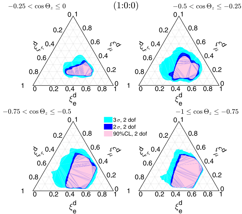
Fig. 4. Allowed regions for the flavor ratios in the presence of NSI in the Earth at 90, 95 and 3\sigma CL for an initial flavor (\xi_e^s : \xi_\mu^s : \xi_\tau^s) = (1 : 0 : 0) . The four triangles correspond to averaging over neutrinos arriving with directions given in the range 0 \geq \cos \Theta_z > -0.25 (upper left), -0.25 \geq \cos \Theta_z > -0.5 (upper right) -0.5 \geq \cos \Theta_z > -0.75 (lower left), and -0.75 \geq \cos \Theta_z \geq -1 (lower right).
