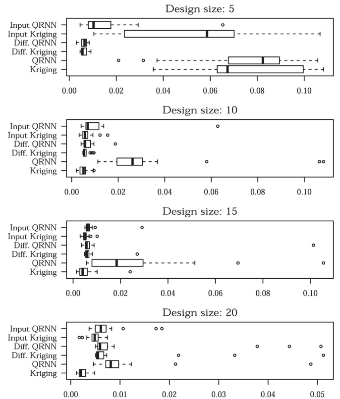
Fig. 9. This plot compares how choosing a different model type (QRNN instead of single-fidelity Kriging) would affect results. Smaller values for the SMSE are better.
