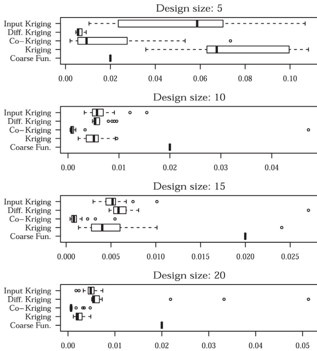
Fig. 7. These plots show how different multi-fidelity methods, based on Kriging, perform in comparison to the coarse function and the single-fidelity Kriging model. Diff. Kriging models the differences between coarse and fine function. Input Kriging uses the coarse function values as an additional input variable. Smaller values for the SMSE are better.
