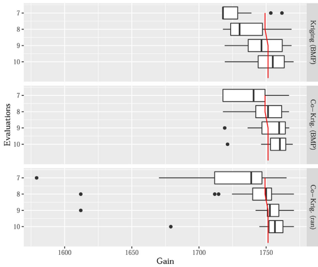
Fig. B.15. Boxplot of 2D optimization performance after each evaluation performed, focusing on best performing methods after the initial six evaluations. Larger values are better. Results are based on 20 repeats of each optimization run. The red line presents the performance of the simplex run with deterministic start point. (For interpretation of reference to color in this figure legend, the reader is referred to the web version of this article.)
