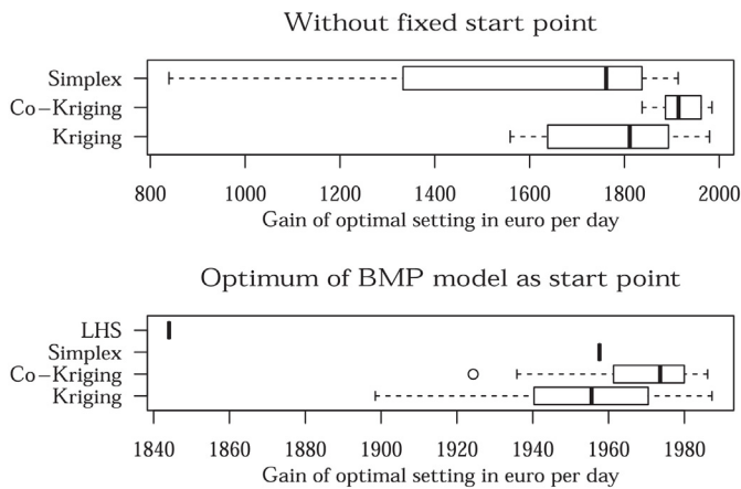
Fig. 11. Boxplot of final results for the 5D optimization with equal number of fine objective function evaluations. Larger values are better. Results are based on 20 repeats of each optimization run. The upper plot shows results where the initial design (or starting guess) was created in a random fashion. For the lower plot, the initial guess (or at least one point in the initial design) was set to the optimum of the coarse objective function.
