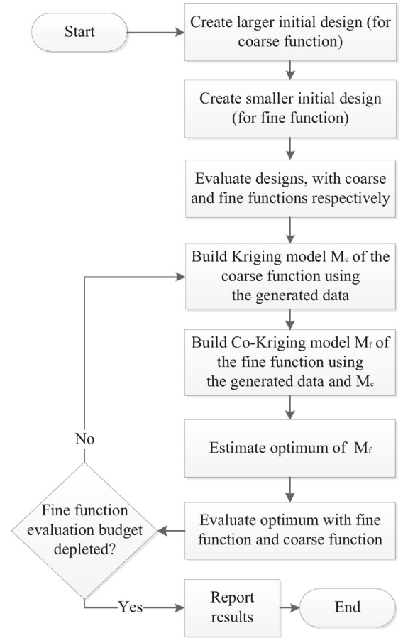
Fig. 1. A flow chart to visualize the algorithmic procedure of optimization with a Co-Kriging surrogate model.
