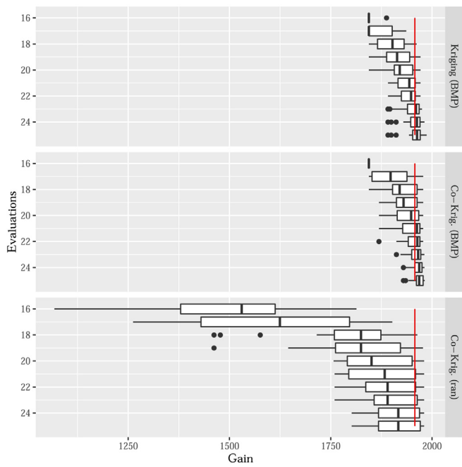
Fig. B.16. Boxplot of 5D optimization performance after each evaluation performed, focusing on best performing methods after the initial 15 evaluations. Larger values are better. Results are based on 20 repeats of each optimization run. The red line presents the performance of the simplex run with deterministic start point. (For interpretation of reference to color in this figure legend, the reader is referred to the web version of this article.)
