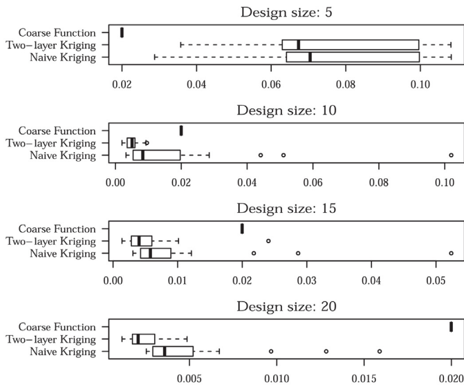
Fig. 6. Again, all plots are based on LHD designs, repeated 20 times. Design sizes are in each header. The two-layer approach models values with and without manure bonus separately. Smaller values are better.
