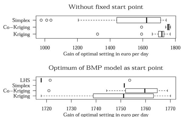
Fig. 10. Final results of 2D optimization. Larger values are better. Results are based on 20 repeats of each optimization run. The upper plot shows results where the initial design (or starting guess) was created in a random fashion. For the lower plot, the initial guess (or at least one point in the initial design) was set to the optimum of the coarse objective function.
