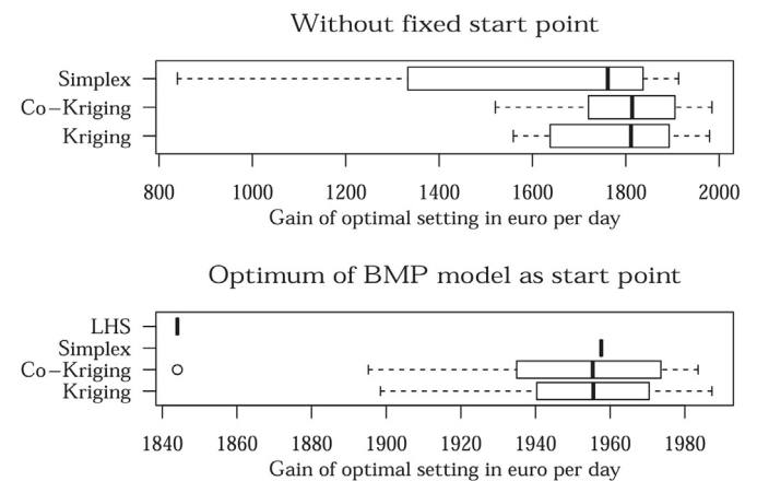
Fig. 12. Boxplot of final results for the 5D optimization with equal runtime. Larger values are better. Results are based on 20 repeats of each optimization run. The upper plot shows results where the initial design (or starting guess) were created in a random fashion. For the lower plot, the initial guess (or at least one point in the initial design) was set to the optimum of the coarse objective-function.
