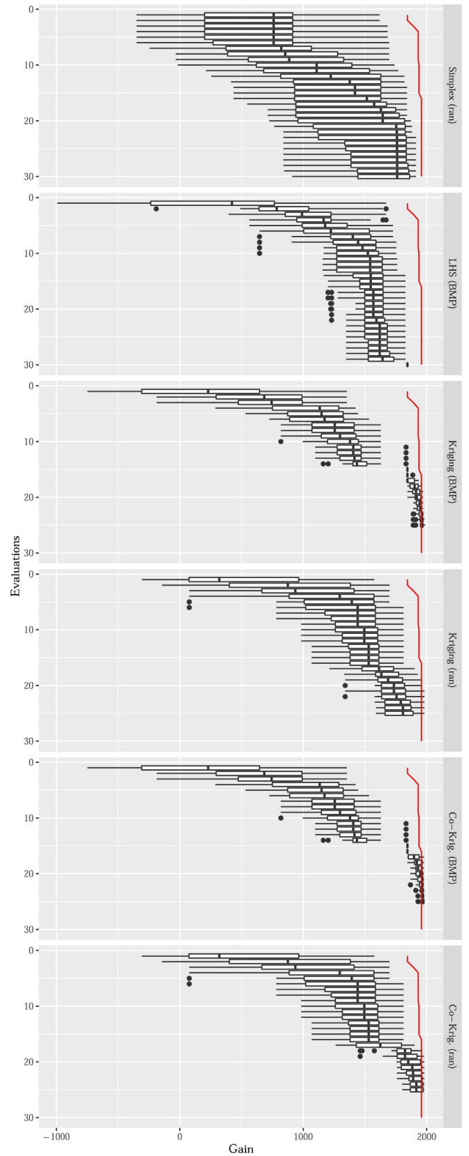
Fig. B.17. Boxplot of 5D optimization performance after each evaluation performed. Larger values are better. Results are based on 20 repeats of each optimization run. The red line presents the performance of the simplex run with deterministic start point. (For interpretation of reference to color in this figure legend, the reader is referred to the web version of this article.)
