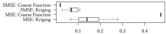
Fig. 5. Depicted are SMSE and MSE of a Kriging model of the fine function as well as the BMP model (coarse function) evaluated by two different error measures. The Kriging model was built based on a LHD of size 5. The process of creating the LHD design was repeated 20 times. Smaller values are better.
