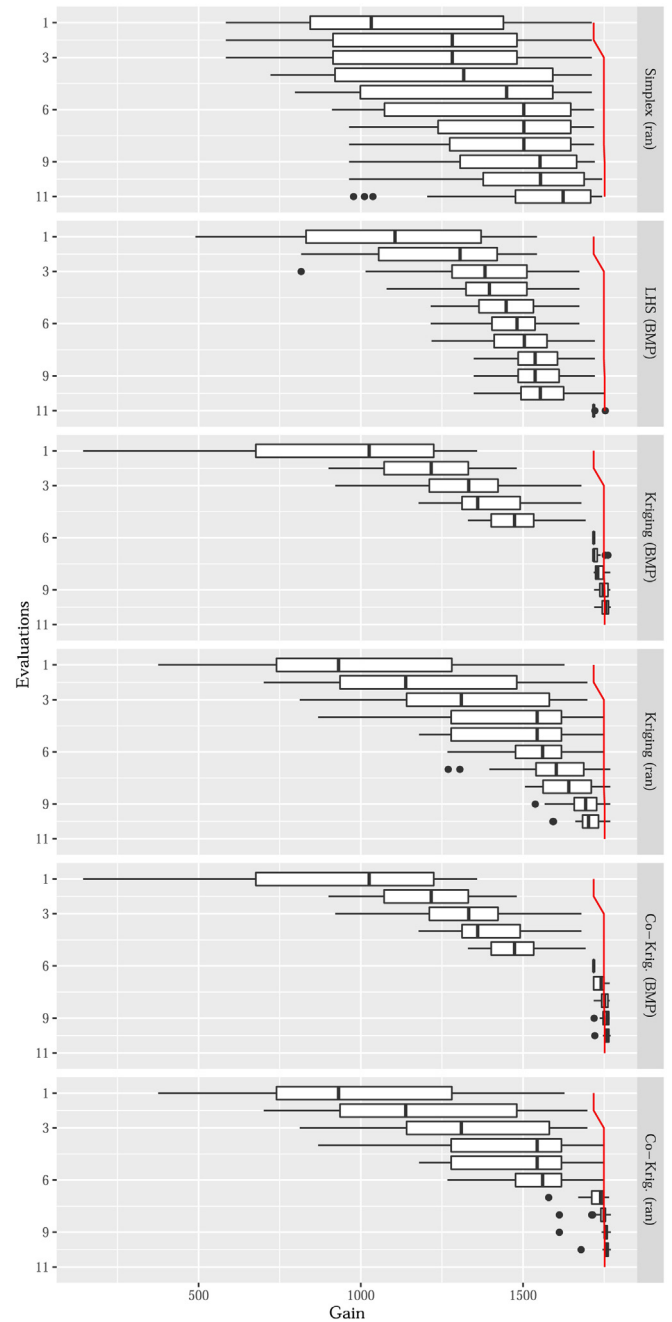
Fig. B.14. Boxplot of 2D optimization performance after each evaluation performed. Larger values are better. Results are based on 20 repeats of each optimization run. The red line presents the performance of the simplex run with deterministic start point. (For interpretation of reference to color in this figure legend, the reader is referred to the web version of this article.)
