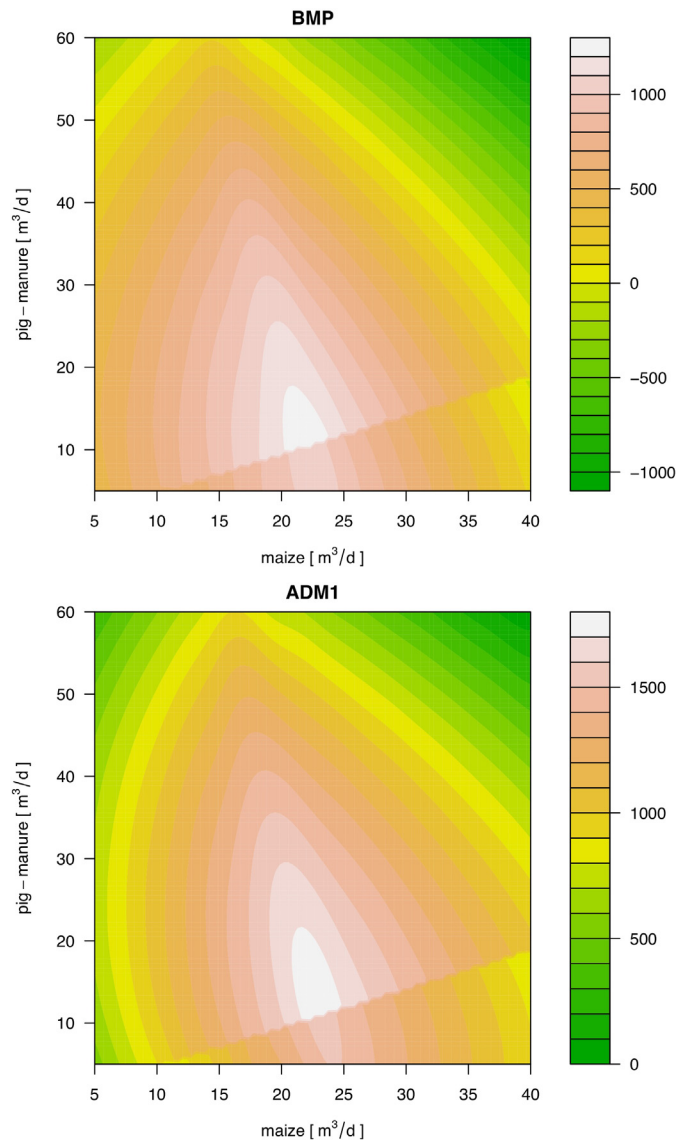
Fig. 3. Contour plots of ADM1 and BMP model, based on 400 samples from a LHD. The two contour plots are both interpolated with Two-layer Kriging, using data from 400 samples generated with LHS. The depicted values are monetary daily gain in Euro, thus larger values are better.
