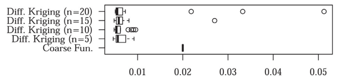
Fig. 8. This plot uses the same data as Fig. 7 but for the Difference-based multi-fidelity approach only. Smaller values for the SMSE are better.
