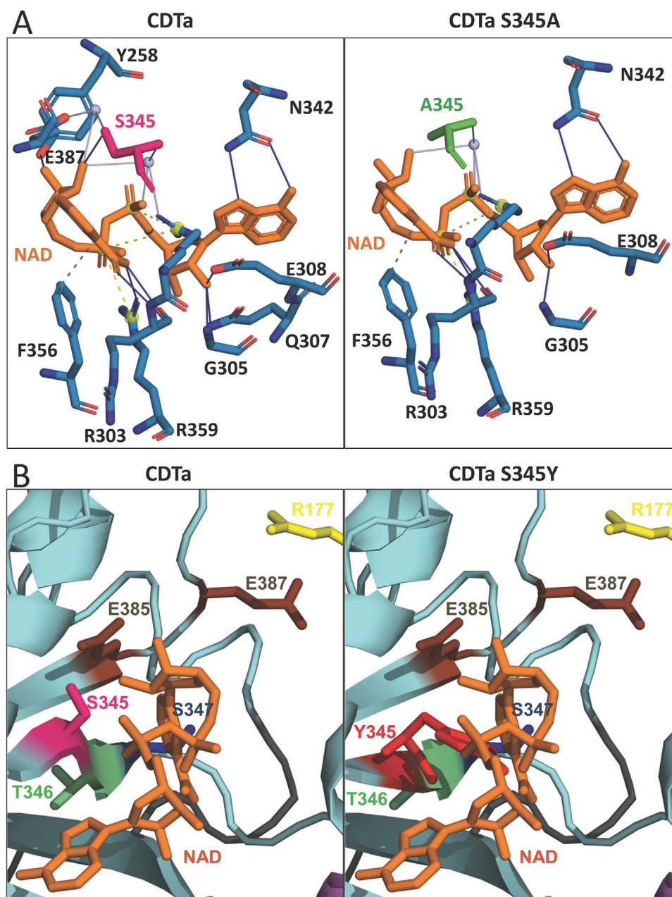
Fig 4. (A) Interaction of rCDTa and CDTa S345A with NAD. Hydrogen bonding, salt bridges, and hydrophobic interactions are shown in blue, grey (dotted), and grey (dotted) lines respectively. Ser-345 is shown in pink and Ala-345 in green. CDTa S345A was generated using Swiss Model [20–23]. Protein ligand profiles were generated using PLIP [24]. (B) Comparison of the active sites of rCDTa and CDTa S345Y. The protein structure for rCDTa has been reported previously [13], PDB accession 2WN7. rCDTa C-terminal region is shown in cyan. NAD cofactor is shown in orange. Residue Arg-177 (ribosylation site) from the modelled Actin is shown in yellow as reference. The active site of S345Y was modelled using Swiss-Model [20–23].
