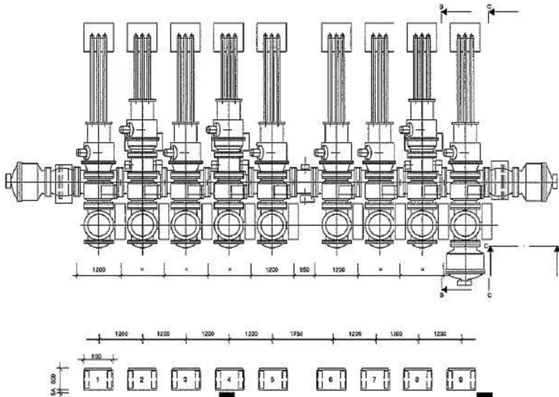
Fig. 2. Layout of switchgears and control panels.
