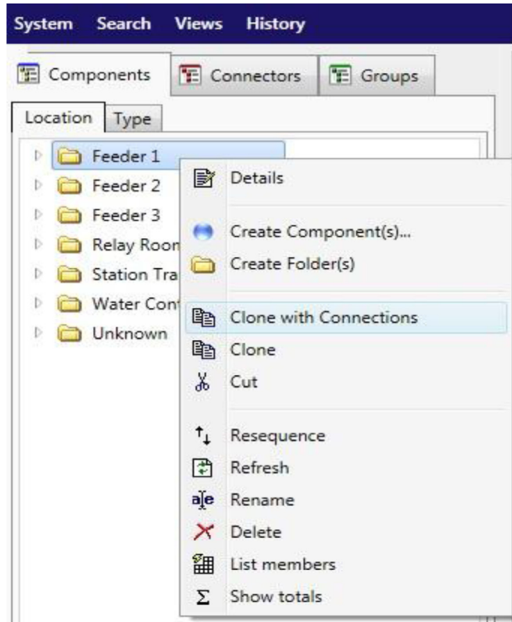
Fig. 4. 'Clone' function.
