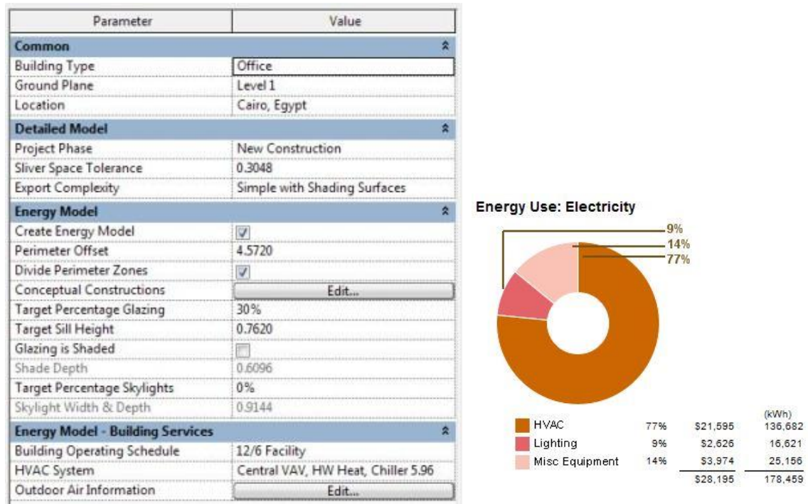
Figure 5 The design options available in Vasari (Left), and a part of the energy analysis report it can create on energy consumption
