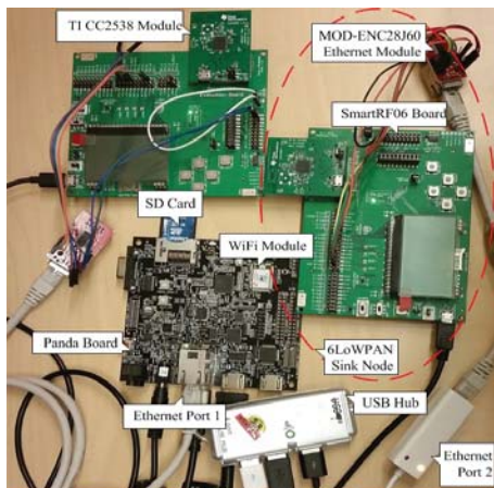
Fig. 5. Gateway Implementation
