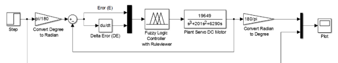
Fig.18. Simulink model for simulating FLC.
