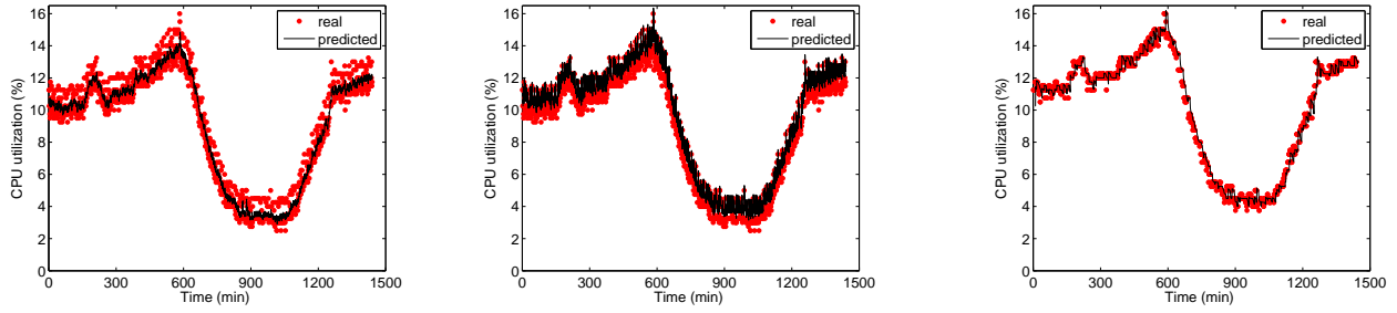
(a) EWMA: \alpha = 0.7, W = 1 (b) FUSD: \uparrow \alpha = -0.2, \downarrow \alpha = 0.7, W = 1 (c) FUSD: \uparrow \alpha = -0.2, \downarrow \alpha = 0.7, W = 8 Fig. 2. CPU load prediction for the DNS server at our university. W is the measurement window.
