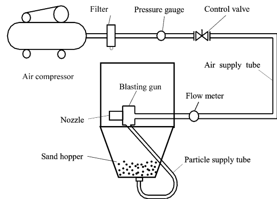
Fig. 1. Schematic diagram of the sand blasting equipment (type GS-6, made in China).
