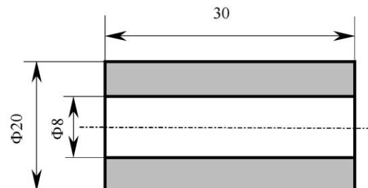
Fig. 2. Geometry and dimensions of the ceramic nozzle.
