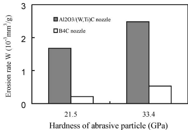
Fig. 10. Variation of nozzle erosion rates with the hardness of the erodent abrasive particles in sand blasting process (erodent abrasive particles: \text{Al}_2\text{O}_3 and SiC, abrasive grain size: 60 mesh).
