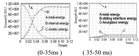
Fig. 4 The energy absorption curve
