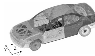
Figure 1 Whole Car finite element model
