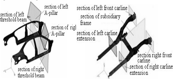
Fig. 7 The section force plane of car model
