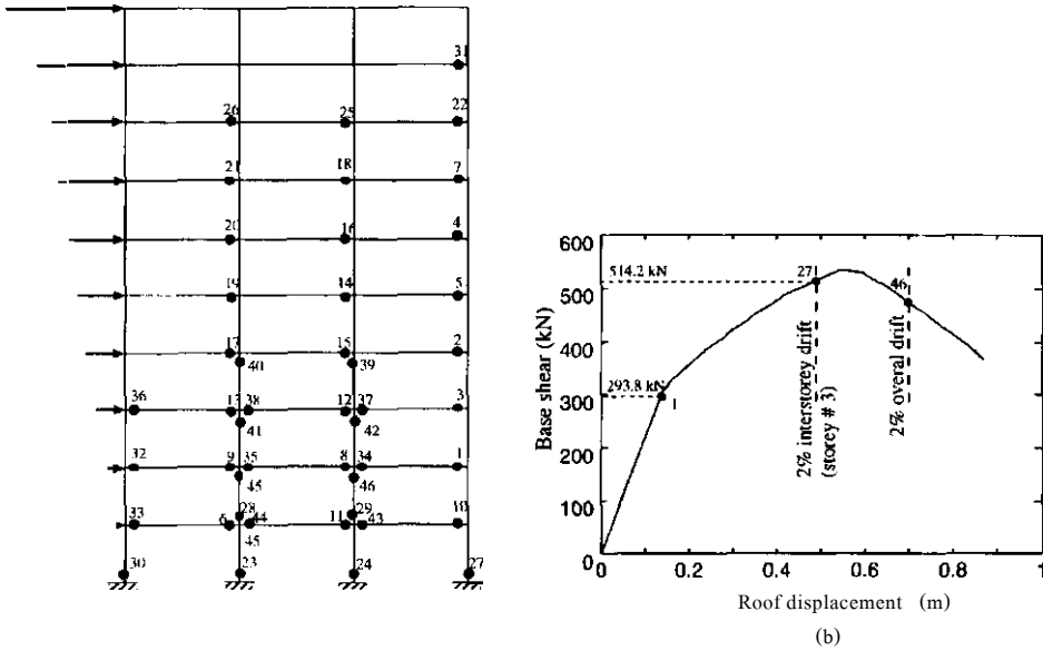
Figure 3: Results of push-over analysis for a 10 storey frame, P- A included, strain hardening modulus = 0; (a) sequence of formation of hinges; (b) base shear versus roof displacement
