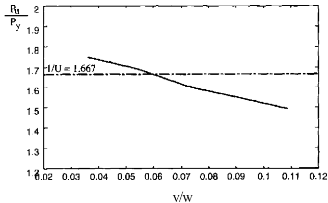
Figure 5: Effect of ratio of earthquake force to gravity force on the reserve strength of a 10 storey building, P-A effect included, 0% strain hardening
