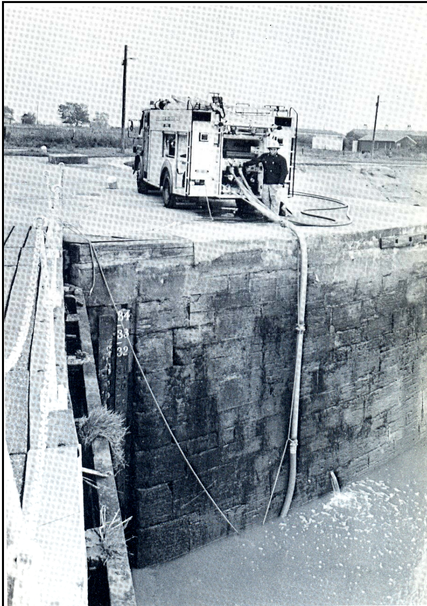
Plate 17. Pump operation involving a deep lift from open water. Note the positioning of the appliance and the lines attached to the suction, one of which is secured to the appliance and the other to the quayside.
