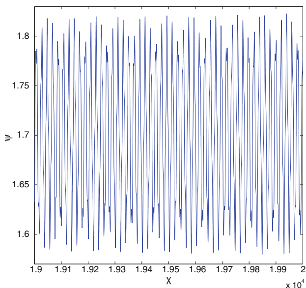
Fig. 8 Quasiperiodicity of \psi based on system (24)
