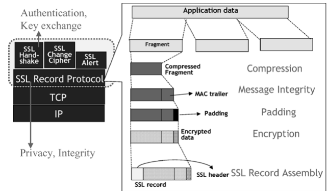
Figure 2. SSL protocol, with an expanded view of the SSL record protocol
