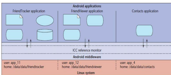
Figure 6. Android security architecture
