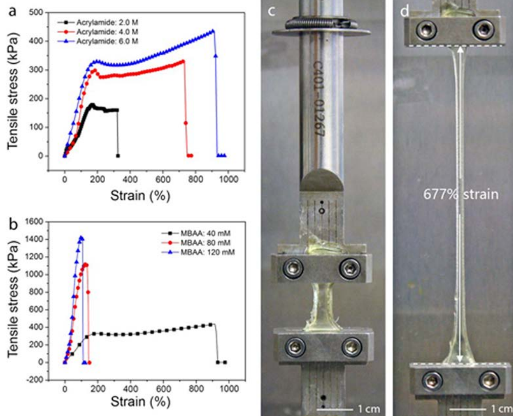
Figure 4. (a) Tensile stress–strain curve of samples with 40 mM MBAA in the first network and different concentrations of acrylamide in the second network. (b) Tensile stress–strain curve of samples with different concentrations of MBAA in the first network and 6.0 M acrylamide in the second network. (c,d) A dogbone with 40 mM MBAA and 6.0 M acrylamide before and after stretching to 677% strain.
