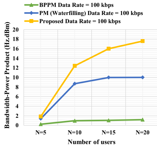
Fig. 6. Bandwidth-Power product with respect to the number of users.
