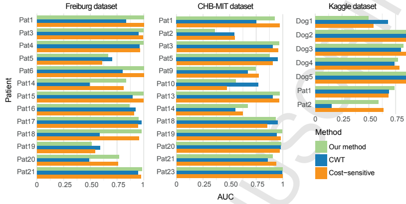
Figure 6: Comparison among our method, the preprocessing step using the continuous wavelet transform (CWT) (Khan et al., 2017), and cost-sensitive learning. AUC, area under the receiver operating characteristic curve; CHB, Boston Children’s Hospital.
