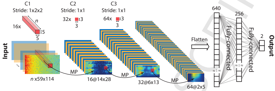
Figure 3: Convolutional neural network architecture. This illustration is applied to the Freiburg Hospital and Boston Children’s Hospital–MIT datasets. For the American Epilepsy Society Seizure Prediction Challenge dataset, the feature sizes are different because of the different recording sampling rate. Short-time Fourier transforms of 30-s windows of raw EEG signals are input. There are three convolution blocks, named C1 , C2 , and C3 . Each block consists of a batch normalization, a convolution layer with a rectified linear unit (ReLU) activation function, and a max pooling layer. For simplicity, max pooling layers are not shown and are noted as MP . For C1 , there are 16 n \times 5 \times 5 kernels, where n is the number of EEG channels, with stride of 1 \times 2 \times 2 . ReLU activation is applied on convolution results before they are subsampled by a pooling over a 1 \times 2 \times 2 region. The same steps are applied in C2 and C3 except the convolution kernel size is 3 \times 3 , stride is 1 \times 1 , and max pooling size is 2 \times 2 . Blocks C2 and C3 have 32 and 64 convolution kernels, respectively. Features extracted by the three convolution blocks are flattened and connected to two fully connected layers with output sizes of 256 and 2, respectively. The former fully connected layer uses a sigmoid activation function, while the latter uses a soft-max activation function. Both of the fully connected layers have a dropout rate of 0.5.
