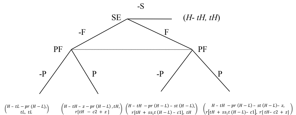
Figure 2: Sequential game with imperfect information and with the specialist's performance.
