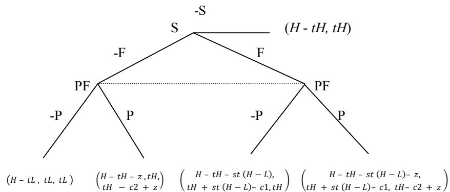
Figure 1: Sequential game with imperfect information and without specialists.
