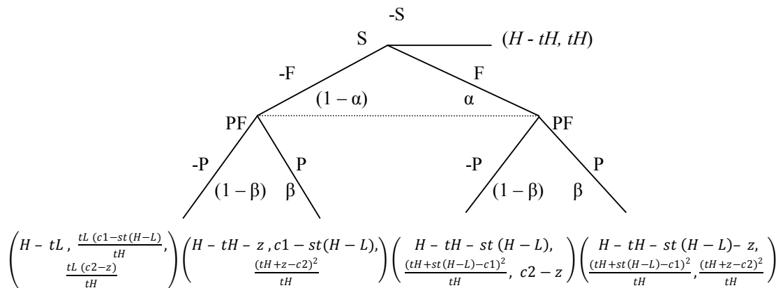
Figure 3: Sequential game with imperfect information and without the specialist's performance - mixed strategies
