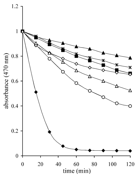
Fig. 2. Rate of \beta -carotene bleaching in control without antioxidant ( \blacklozenge ), oregano essential oil ( \blacksquare ), CHO fraction ( \blacktriangle ), phenolic compounds fraction ( * ), CH fraction ( \circ ), thymol ( \diamond ) and carvacrol ( \triangle ). The concentration of the total essential oil, its fractions and pure compounds was 4 g/l.
