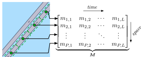
Figure 2: Illustration of the time-space matrix model
