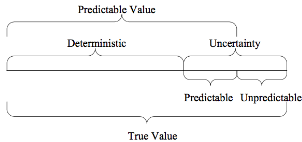
Figure 4: Predictable and unpredictable components of a variable [67]
