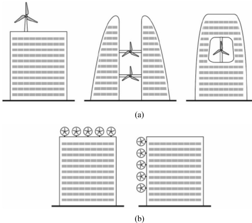
Fig. 6. Possible installation of BIWT: (a) Large size wind turbines and (b) System of small size wind turbines (Park et al., 2015).
