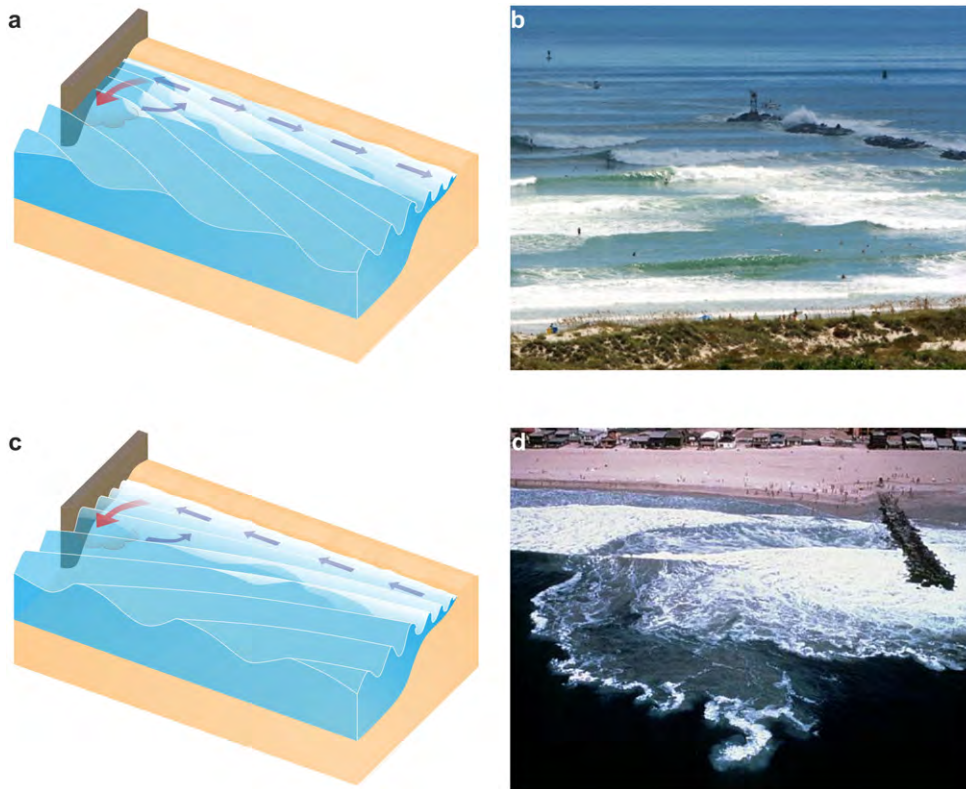
Fig. 10. Examples of boundary rip currents: a) schematic of a shadow rip current in the lee of an obstacle (upwave side); b) shadow rip current against Ponce Inlet Jetty, Florida, US ( www.bv.com ); c) deflection rip current adjacent to obstacle on downwave side of beach; d) deflection rip current at Newport Beach, California, US ( http://www.oceregister.com/articles/rip-130324-current-never.html ).
