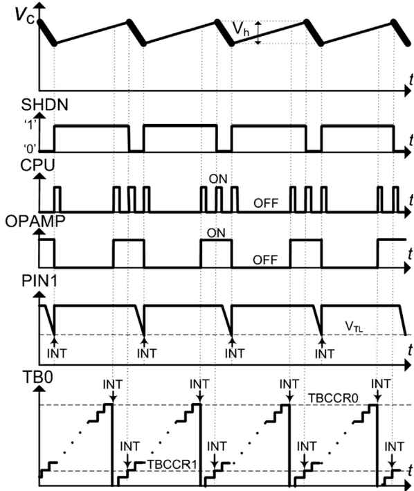
Fig. 9. MPPT timing diagram showing the activity of CPU, timer B0 (TB0), OPAMP and switching converter.
