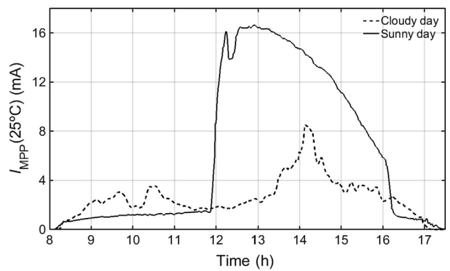
Fig. 15. I_{MPP}(25^\circ\text{C}) measured during a sunny and a cloudy day.
