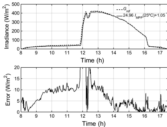
Fig. 18. Comparison between the measured and the reference irradiance during a sunny day.
