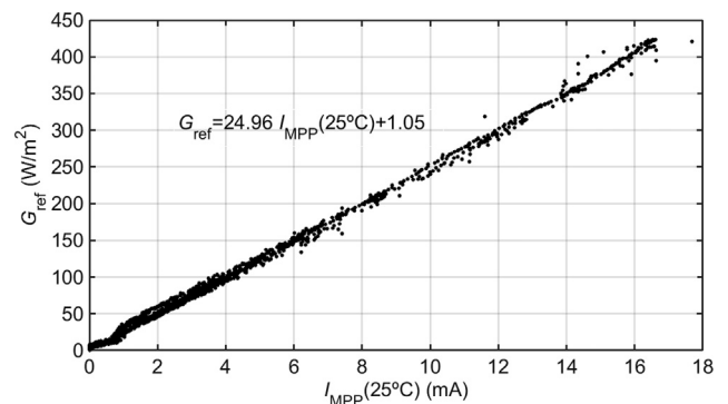
Fig. 16. G_{ref} versus I_{MPP}(25^\circ\text{C}) obtained during several days and the resulting linear regression.
