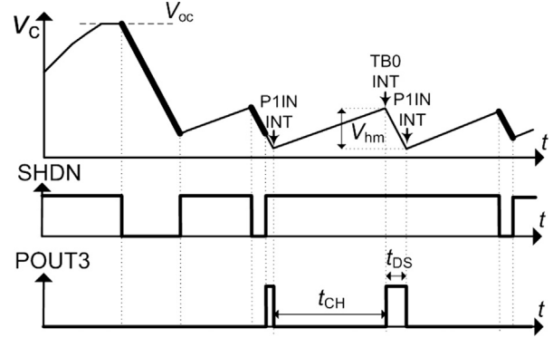
Fig. 11. Timing diagram of the activity to measure I_{MPP} by applying (4).
