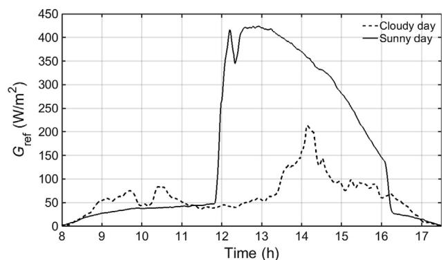
Fig. 14. Irradiance measured by a HD52.3DP147 pyranometer during a sunny and a cloudy day.
