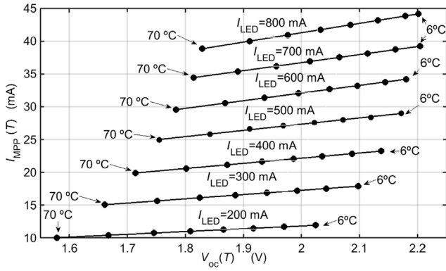
Fig. 5. Temperature dependence of I_{MPP} for SLMD121H04.
