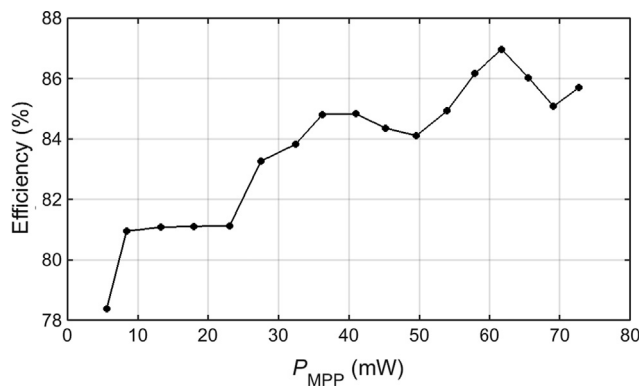
Fig. 13. Efficiency ( \eta ) of the energy harvester versus the incoming power of the PV panel.
