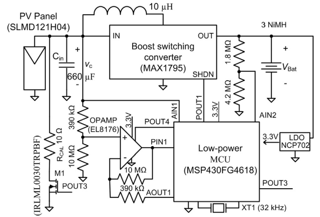
Fig. 8. Circuit diagram of the MPPT system implemented.
