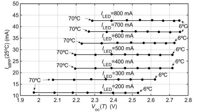
Fig. 7. Temperature compensation of I_{MPP} .
