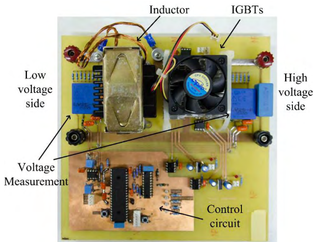
FIGURE 11. The experimental bidirectional DC-DC converter.
