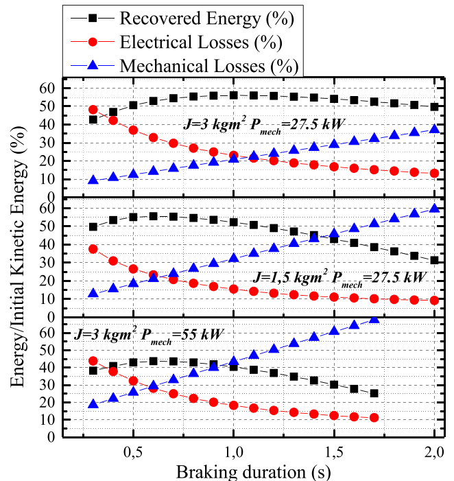
FIGURE 8. Search algorithm results for different load conditions and different load of inertia values.
