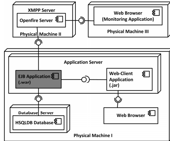
Figure 4. ARAMIS Deployment Diagram
