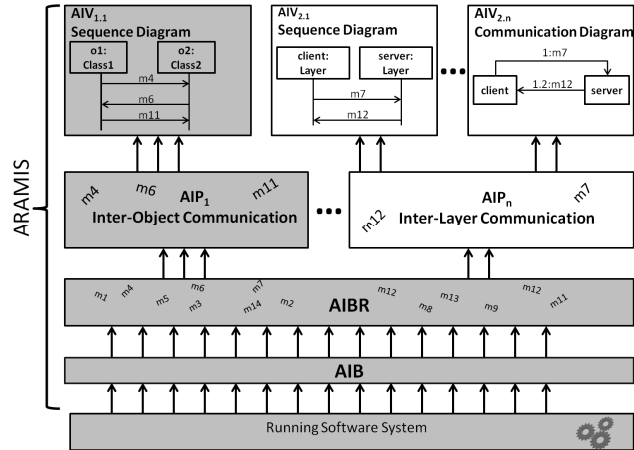
Figure 1. ARAMIS – Conceptual Overview ([7])
