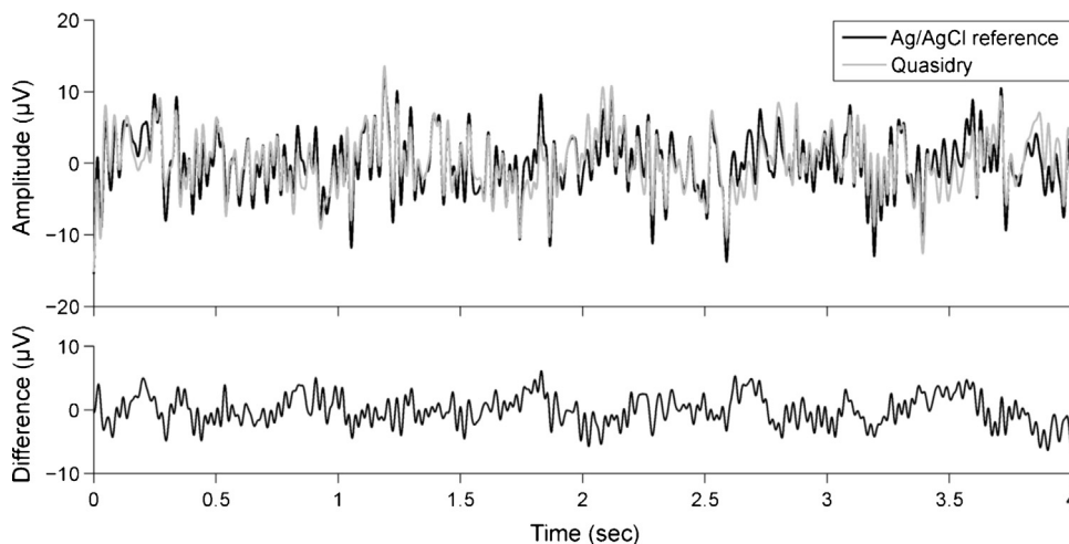
Fig. 10. 4 s of resting EEG signal for reference Ag/AgCl and quasi-dry electrodes at the O1 position, in time domain.
